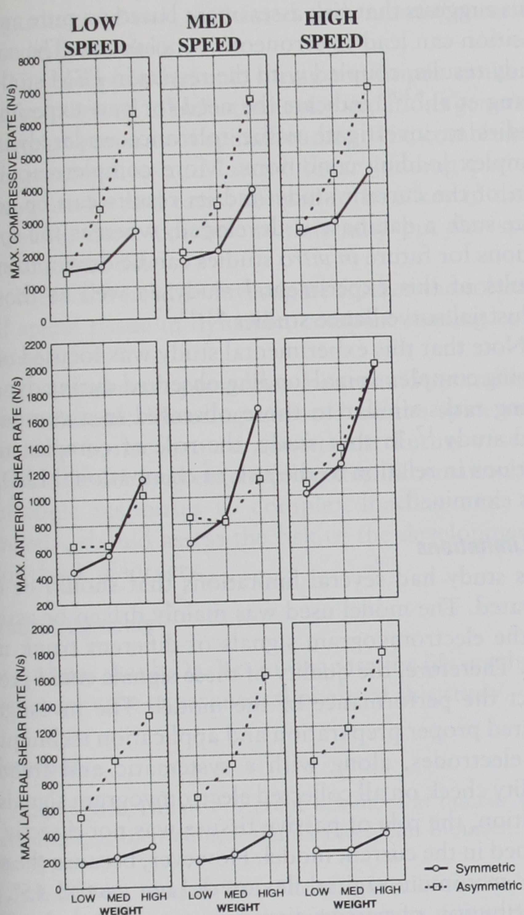
Figure 7. Average maximum loading rate in all spinal loading directions under each weight-speed combination for the symmetric and asymmetric lifts. Note that the high weight-high speed asymmetric condition is considered a high risk situation, whereas the low weight-low speed symmetric condition would be considered a low risk situation.
