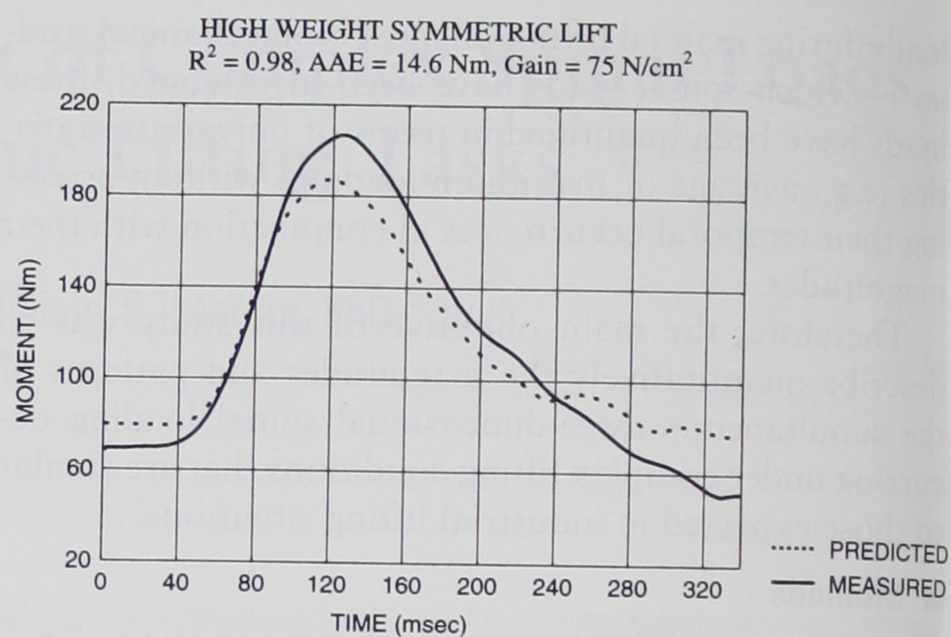
Figure 2. Measured extension moment versus the predicted moment of a typical symmetric lift.
