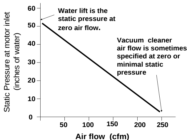
Figure A. Illustration of pump or fan curve
