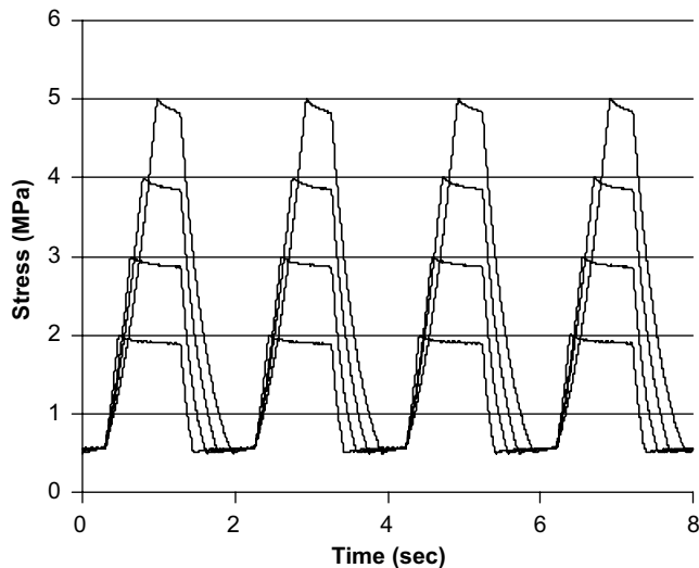
Fig. 1. Loading profile over four cycles of load for tendons loaded between 0.5 MPa and a peak stress of 2, 3, 4 or 5 MPa.
