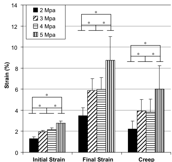
Fig. 2. Mean ( \pm SD) initial strain, final strain and creep in tendons cyclically loaded to a peak stress of 2, 3, 4, 5 MPa for 18 h. Cyclic loading to higher peak stresses led to greater initial strain, final strain and creep. ( n = 10 , *p < 0.05 ).
