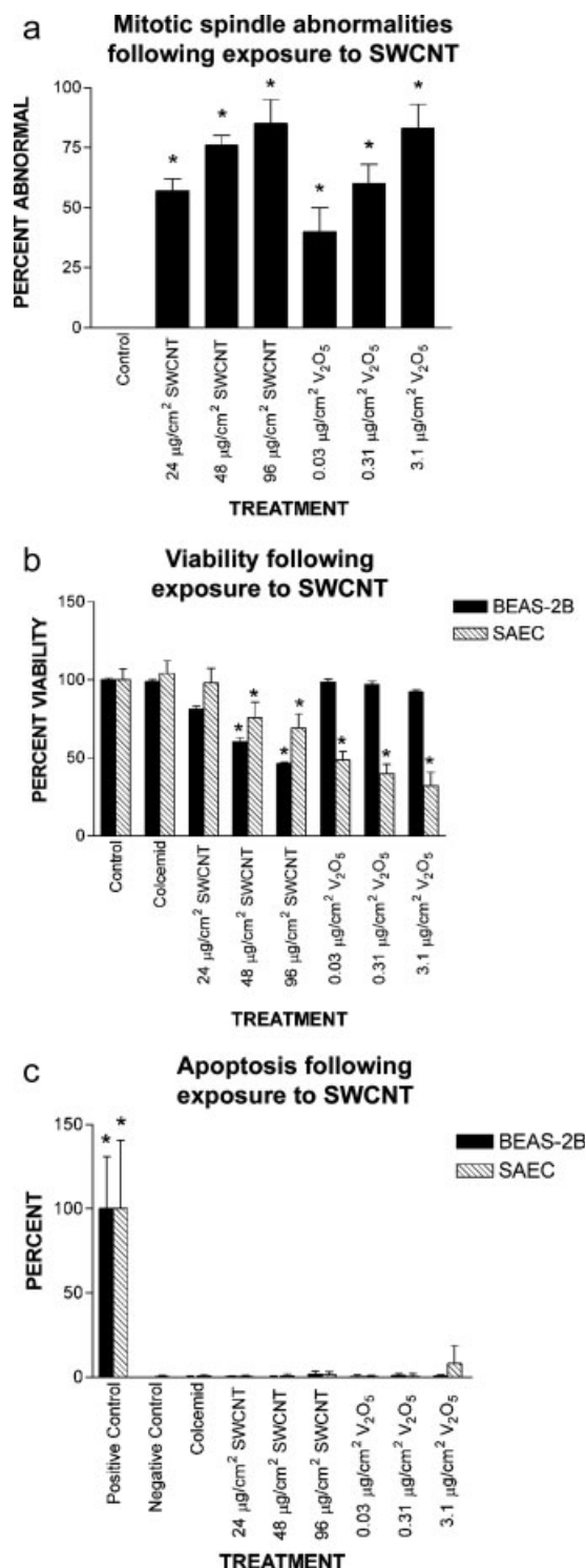
Fig. 1. Toxicity of SWCNT. (a) Figure 1 shows the percentage of cells that were observed with mitotic spindle abnormalities. The solid bars indicate the level of apoptosis in control and exposed BEAS-2B. Mitotic spindle abnormalities are expressed as a percent of total mitotic figures. The abnormalities included monopolar, tripolar, and quadrapolar mitotic spindles, and nanotubes displacing portions of the mitotic spindle. * indicates significantly different from the unexposed control cells at P < 0.001 . (b) The bar graph shows viability of BEAS-2B and SAEC cells following exposure to SWCNT or \text{V}_2\text{O}_5 . The solid bars indicate the level of viability in control and exposed BEAS-2B. The hatched bars indicate the level of apoptosis in the exposed SAEC. SWCNT exposure resulted in reduced viability in the Alamar Blue assay in the SAEC and the BEAS-2B at 48 and 96 \mu\text{g}/\text{cm}^2 compared to control cells. The exposure to \text{V}_2\text{O}_5 resulted in reduced viability in SAEC-treated cells at all doses; however, a reduction in viability was not observed in the \text{V}_2\text{O}_5 -treated BEAS-2B cells. *Indicates statistical significance at P < 0.001 . (c) The solid bars indicate the percentage of apoptotic cells in control and exposed BEAS-2B. The hatched bars indicate the percentage of apoptotic cells in control and exposed SAEC. The DNase-treated positive control showed significant apoptosis in the BEAS-2B and the SAEC; however, exposure to SWCNT or \text{V}_2\text{O}_5 did not induce apoptosis.
