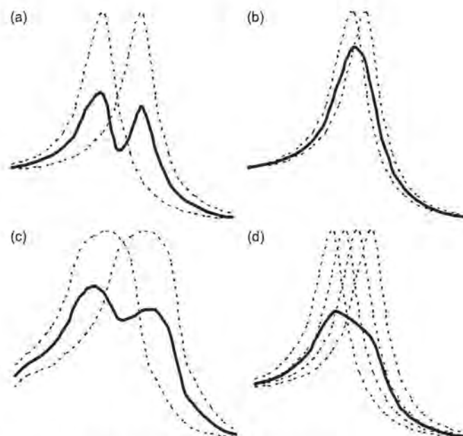
Fig. 1. Factors affecting the arithmetic averaging effects: (a) comparison of the original responses and the averaged response; (b) effect of the distance between peaks or natural frequencies; (c) effect of the damping of the system on the kurtosis of the response; and (d) effect of the number of subjects (----- assumed original data; ——— averaged data).
