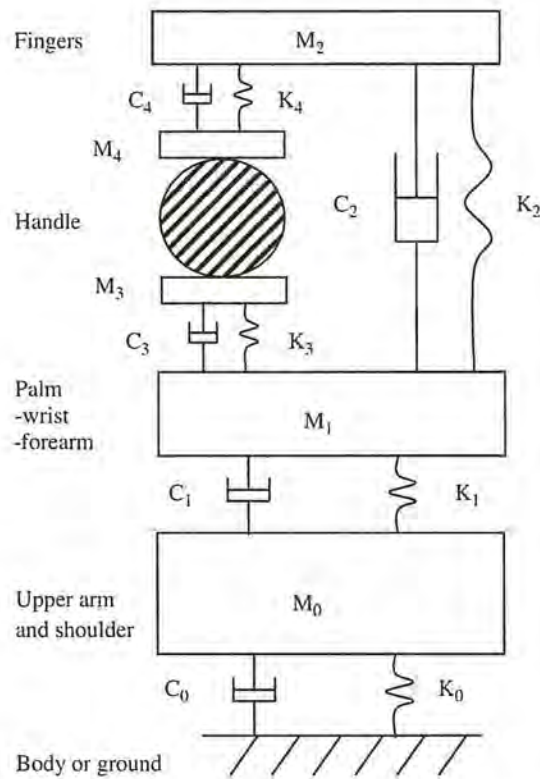
Fig. 2. A 5-DOF model of the hand-arm system [14].
