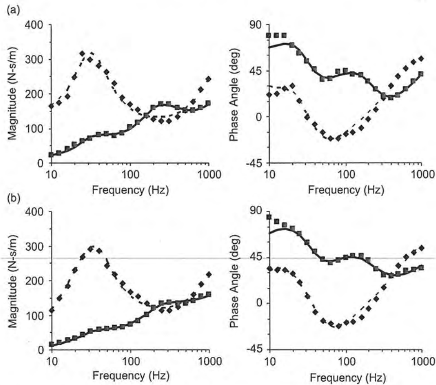
Fig. 6. Comparisons of the laboratory-measured mean responses and the modeling responses calculated using the conventional modeling method [14,18,19]: (a) with the six-subject data and (b) with the eight-subject data (◆ palm laboratory-measured mean response; ----- palm modeling response; ■ fingers laboratory-measured mean response; ——— fingers modeling response).
