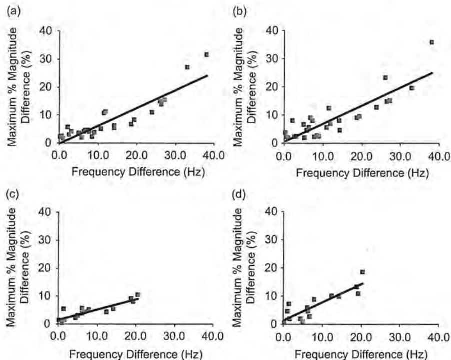
Fig. 8. The relationship between the second natural frequency difference ( \Delta f = f_{2\_Subject\_i} - f_{2\_Subject\_j} , i \neq j ) of two subjects and the maximum error of the arithmetically averaged response in the frequency range of 16 to 1000 Hz: (a) palm maximum percent magnitude error from the eight-subject data; (b) fingers maximum percent magnitude error from the eight-subject data; (c) palm maximum percent magnitude error from the six-subject data; and (d) fingers maximum percent magnitude error from the six-subject data. (■ the relationship raw data; — trendline).
