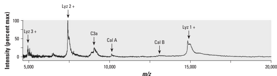
Figure 3. Protein identification for SELDI-TOF peaks. max, maximum. The predominant peaks identified by MS/MS or MS E in BALF obtained at 24 hr postexposure to DEP are labeled with the corresponding protein: anaphylatoxin C3a (C3a), calgranulin A (Cal A), calgranulin B (Cal B), or lysozyme (Lyz). The three different charge states observed for lysozyme are indicated.
