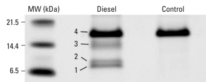
Figure 2. Gel electrophoresis of extracted BALF obtained at 24 hr posttreatment from a control rat (PBS instilled) and a rat exposed intratracheally to 50 mg of DEP/kg body weight. The four numbered bands in the diesel lane were excised and analyzed by LC/MS.
