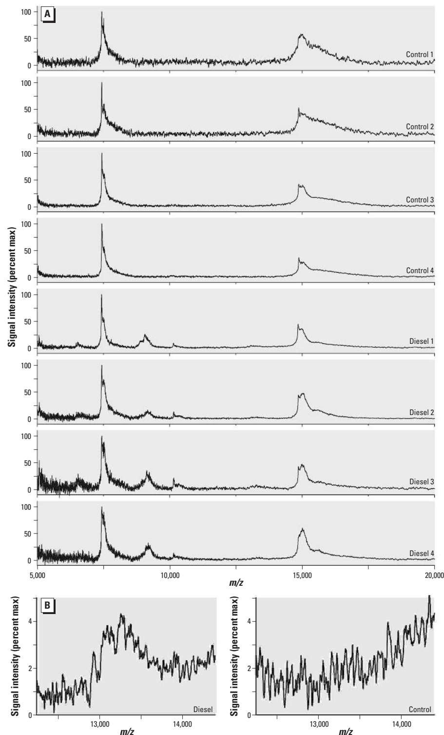
Figure 1. (A) SELDI-TOF mass spectra of BALF obtained at 24 hr post-treatment from four control rats (PBS instilled) and four rats exposed intratracheally to 50 mg DEP/kg body weight and (B) a zoomed view of two spectra generated by averaging the data from the four control or four exposed replicates. max, maximum. Peaks at 9,100 and 10,100 are detected only in the spectra from the exposed samples. The peak near 13,100 is also present only in exposed samples but is undoubtedly only above baseline when multiple spectra are averaged.
