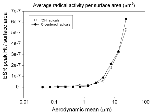
Fig. 4. Free radical activity per unit particle surface area. Both •OH and carbon radicals showed good surface area correlation for ultrafine and fine sizes however, underestimation of true particle surface area or particle bounce may have influenced the coarse particle results.
