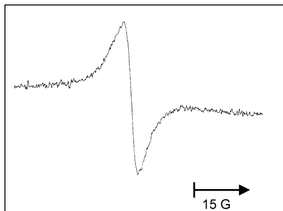
Fig. 1. A typical ESR spectrum of the carbon radical recorded from a dry filter measurement. No change in spectral intensity was observed over a 3-day period. ESR settings were center field, 3490 G; scan width, 100 G; time constant, 0.40 s; modulation amplitude, 1 G; receiver gain, 6.32 \times 10^4 ; frequency, 9.828 GHz; power, 100 mW.
