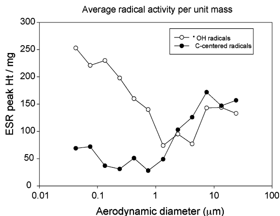
Fig. 3. Free radical activity per unit particle mass. Radical strength of •OH was greatest per unit mass in the smaller particle sizes, while carbon radicals were stronger per unit mass in the coarser particles.
