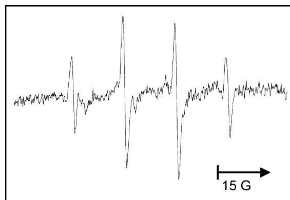
Fig. 2. The generation of short-lived \bullet\text{OH} radicals by wildland smoke upon reaction with \text{H}_2\text{O}_2 . ESR spectrum recorded 3 min after reaction was initiated in PBS (pH 7.4) containing \text{H}_2\text{O}_2 [1 mM] and DMPO [100 mM] vortexed for 1 min with the filter. ESR settings were center field, 3490 G; scan width, 100 G; time constant, 0.40 s; modulation amplitude, 1 G; receiver gain, 6.32 \times 10^4 ; frequency, 9.828 GHz; power, 100 mW.
