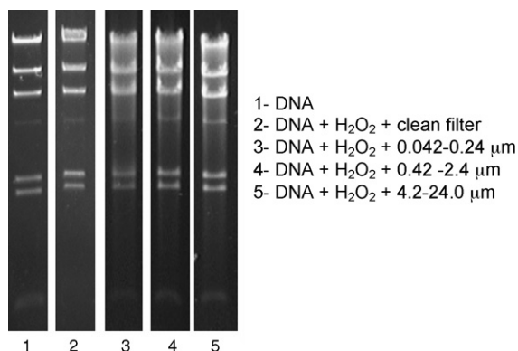
Fig. 9. DNA strand breaks induced by wildfire smoke. Lane 1, \lambda Hind III digested DNA alone; lane 2, DNA + H 2 O 2 [1 mM] + clean control filter suspension; lane 3, DNA + H 2 O 2 [1 mM] + 0.042–0.24 μm wildfire filter suspension [100 μg/ml]; lane 4, DNA + H 2 O 2 [1 mM] + 0.42–2.4 μm wildfire filter suspension [100 μg/ml]; lane 5, DNA + H 2 O 2 [1 mM] + 4.2–24.0 μm wildfire filter suspension [100 μg/ml].
