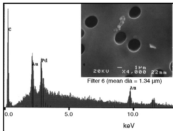
Fig. 6. Elemental particle profile and electron micrograph of particles on sixth filter stage (median particle diameter 1.34 \mu\text{m} ). Smaller particles show a different profile than the larger fraction containing carbon, which could be the result of combustion. The clumping of the smaller particles can also be observed.
