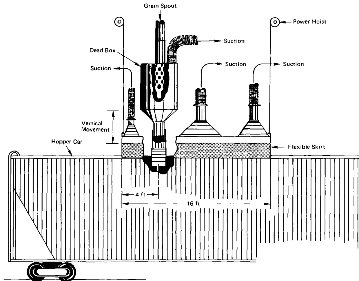
FIGURE 6-10 Combination deadbox with suction hood.
