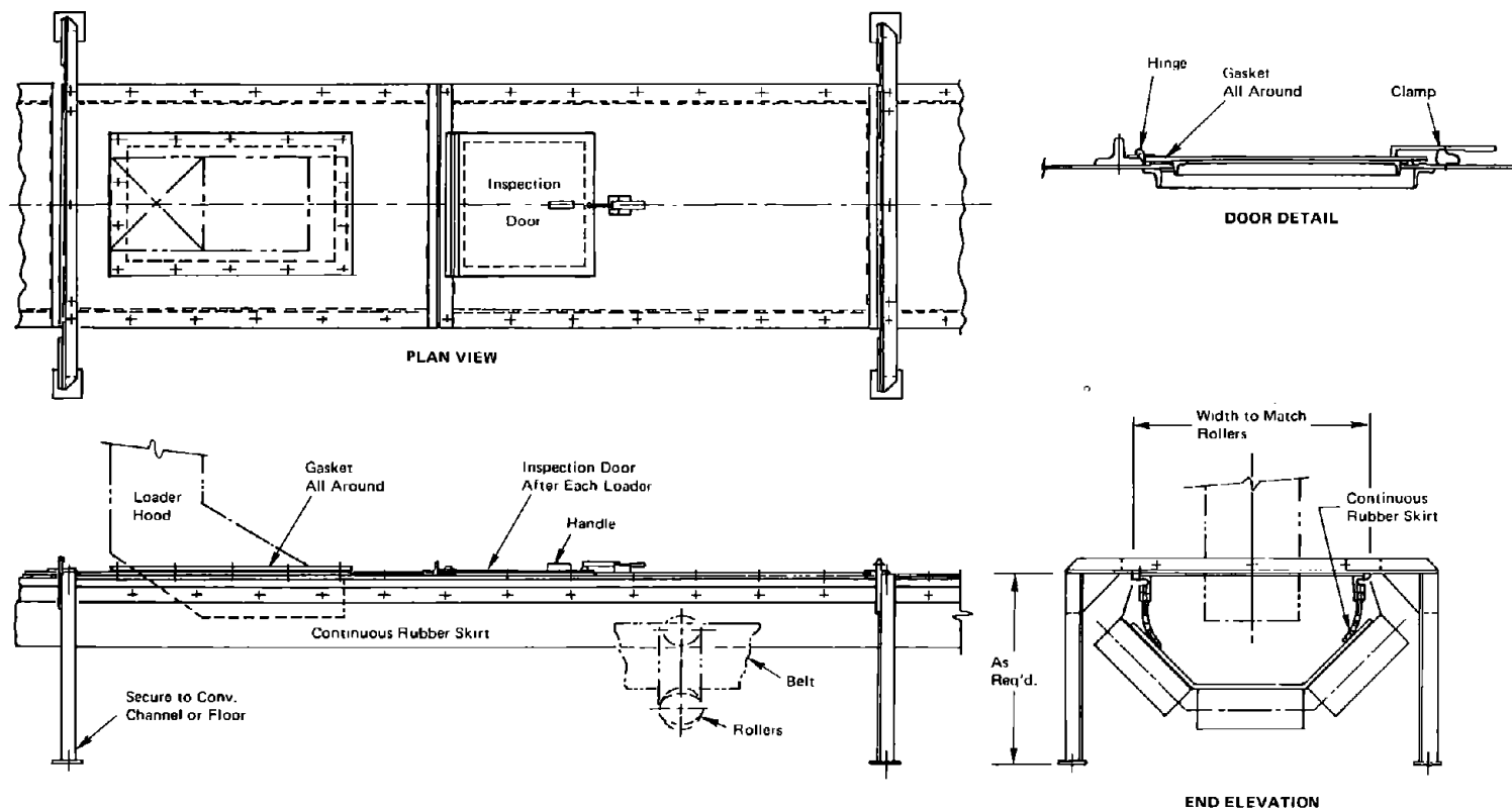
FIGURE 3-4 Continuous belt hood.
