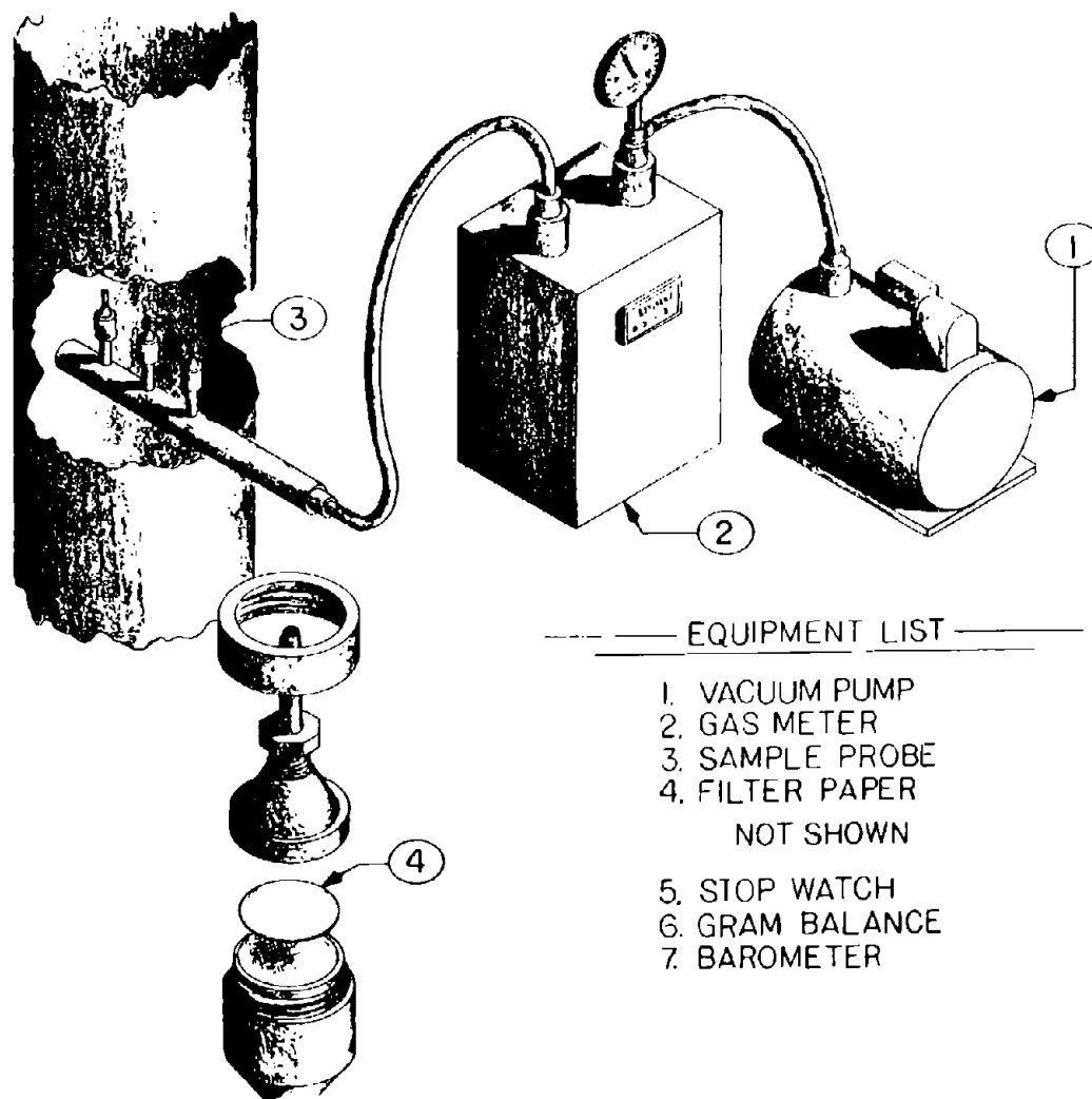
FIGURE C-2 Air flow schematic for sampling procedure.
