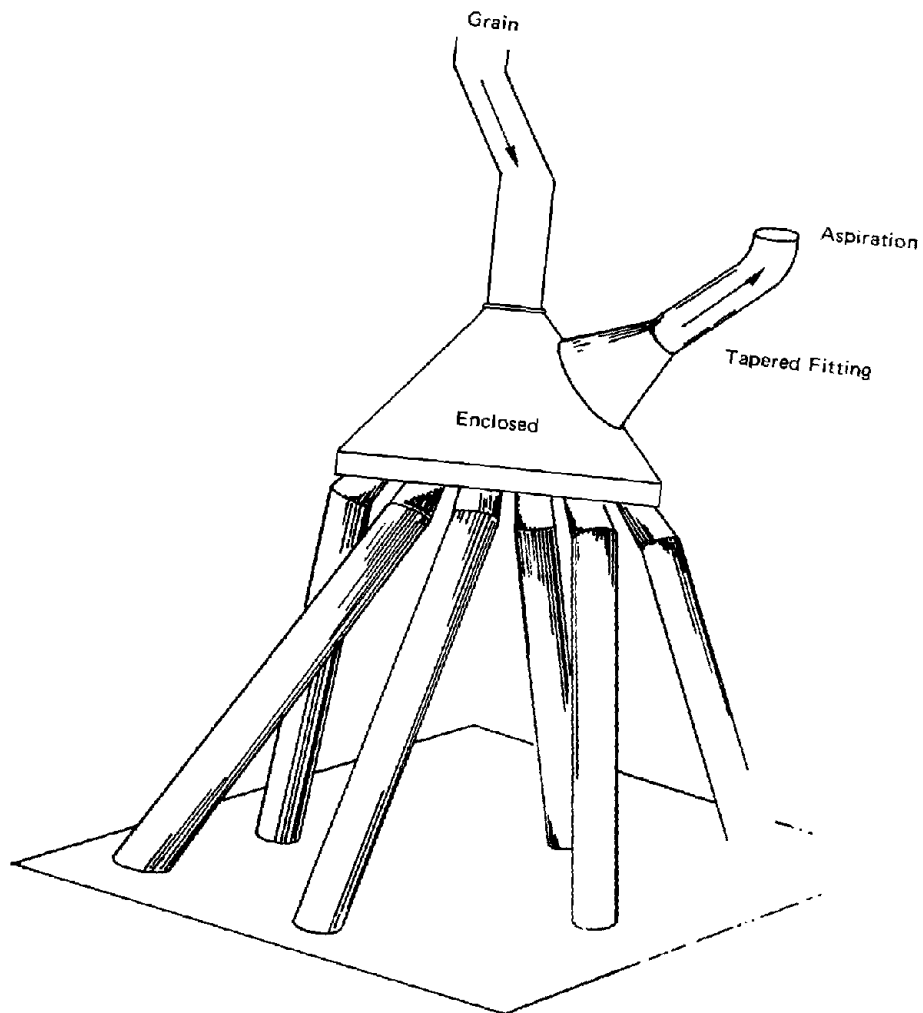
FIGURE 6-6 Enclosed distributor dust control system.
