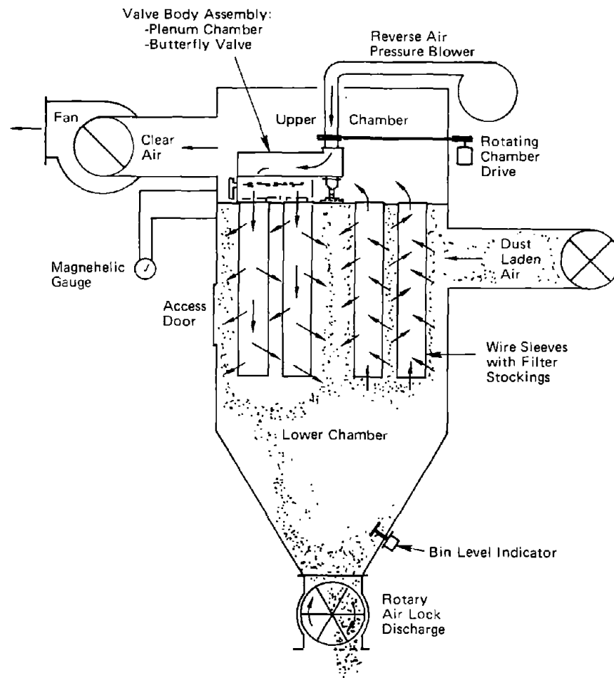
FIGURE 4-1 Typical fabric filter.
