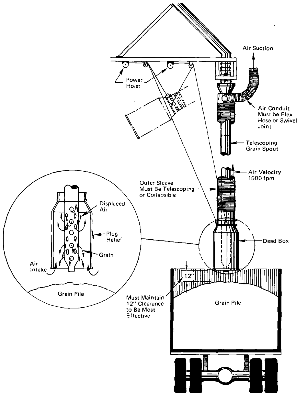
FIGURE 6-9 Retractable spout deadbox for truck load-out.
