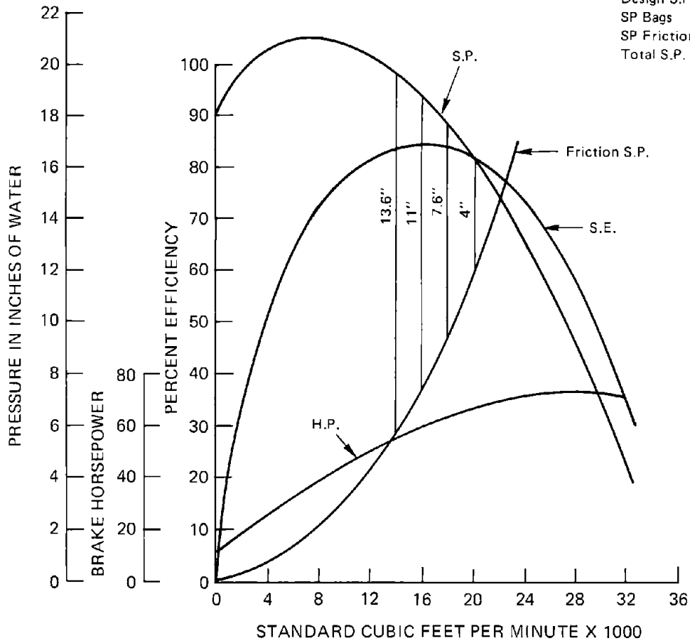
FIGURE 5-5 Typical fan performance chart.
