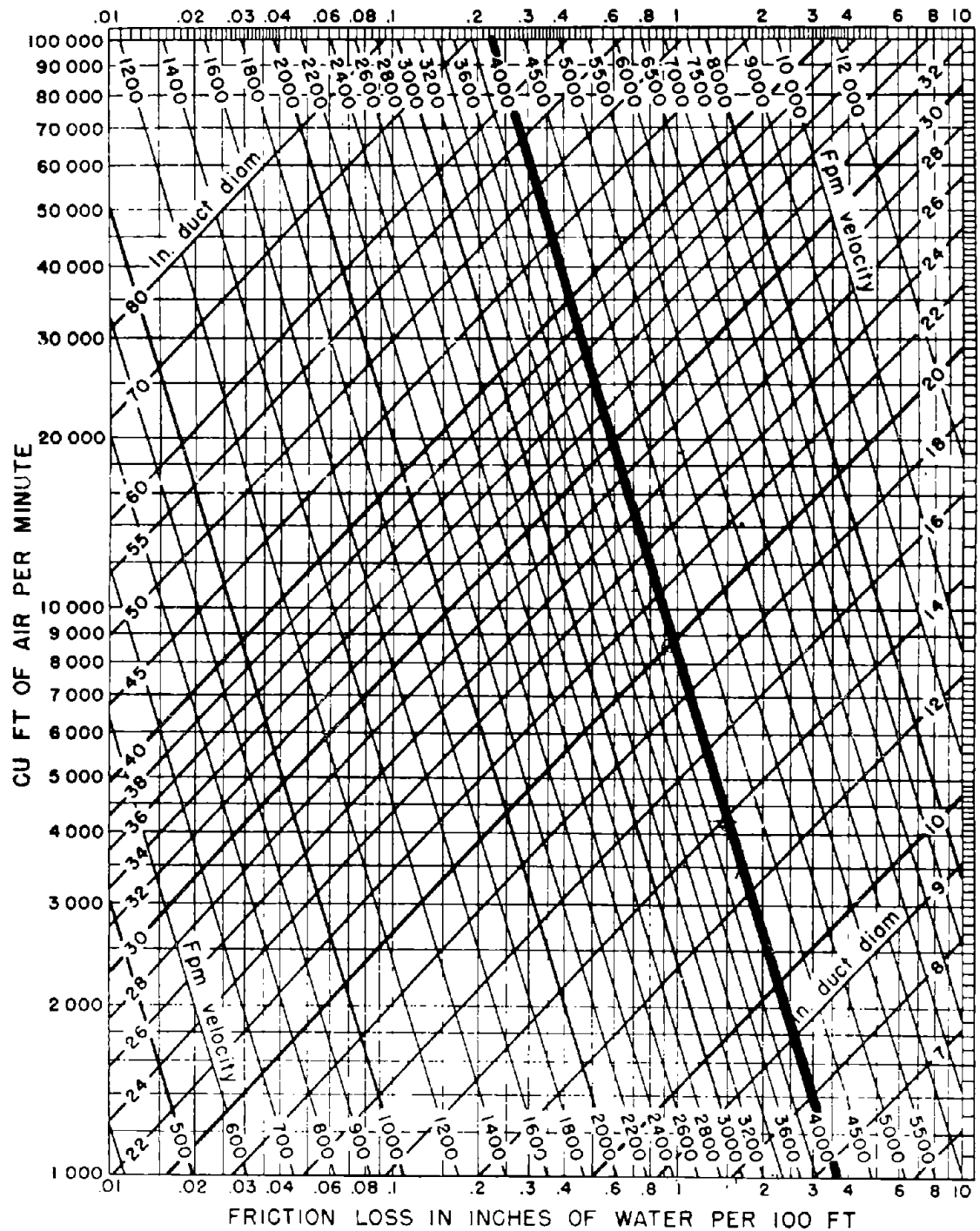
FIGURE 3-7 Tube sizing chart. (Friction of air in straight ducts for volumes of 1000 to 100,000 cfm.)
