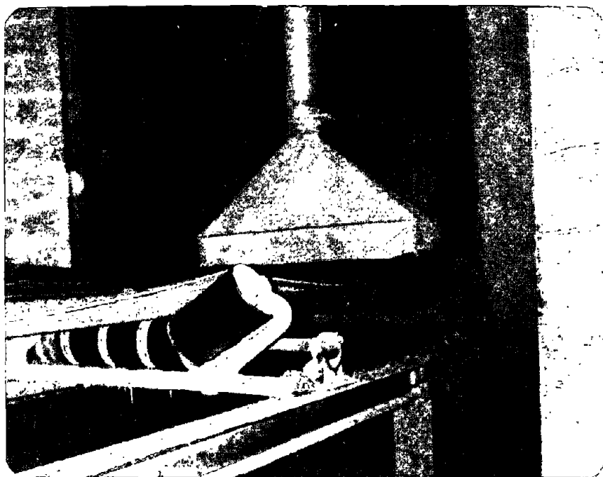
b) Hood situated too far from belt and is not skirted.
