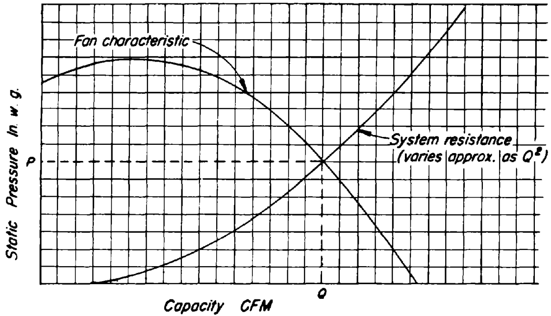
FIGURE 5-3 Typical point of rating. (from "Industrial Ventilation", 16th Edition, 1980)
