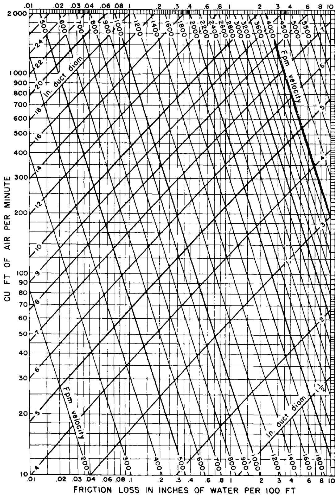
FIGURE 3-6 Tube sizing chart. (Friction of air in straight ducts for volumes of 10 to 2000 cfm.)
