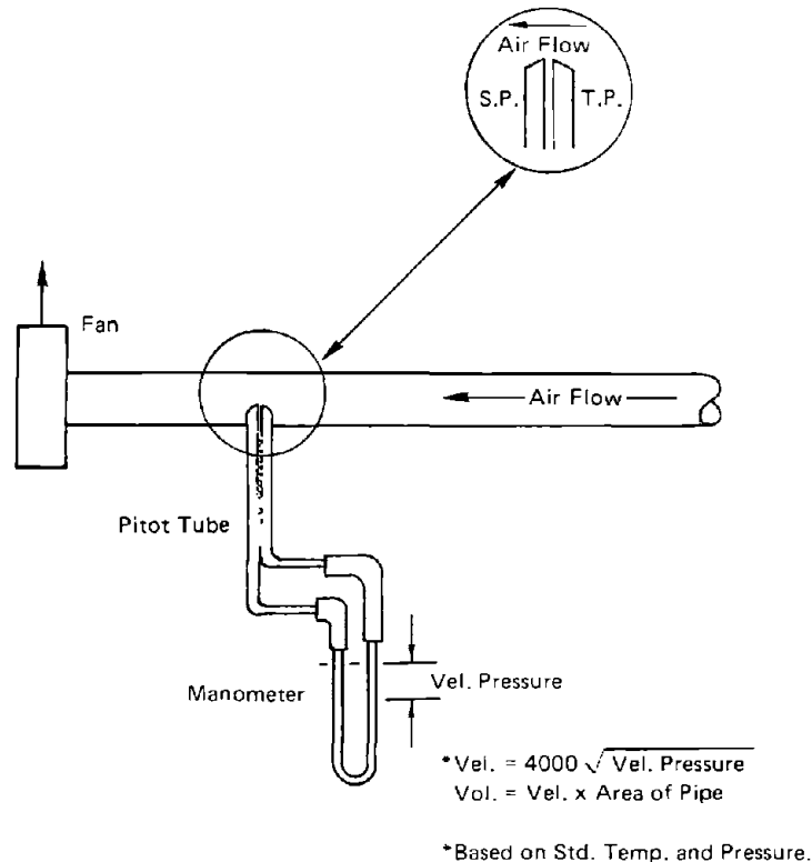
FIGURE 8-4 Pitot tube. The pitot tube, an instrument for measuring velocity pressure, consists of two tubes joined together as shown. Special pitot tubes are required for measuring air flow in a pipe containing dust. The standard ASME tube is unsatisfactory because the holes in the tube plug with dust quickly. The pitot tube is inserted in the pipe at right angles to the air flow and a traverse is made to get the average velocity pressure reading.
