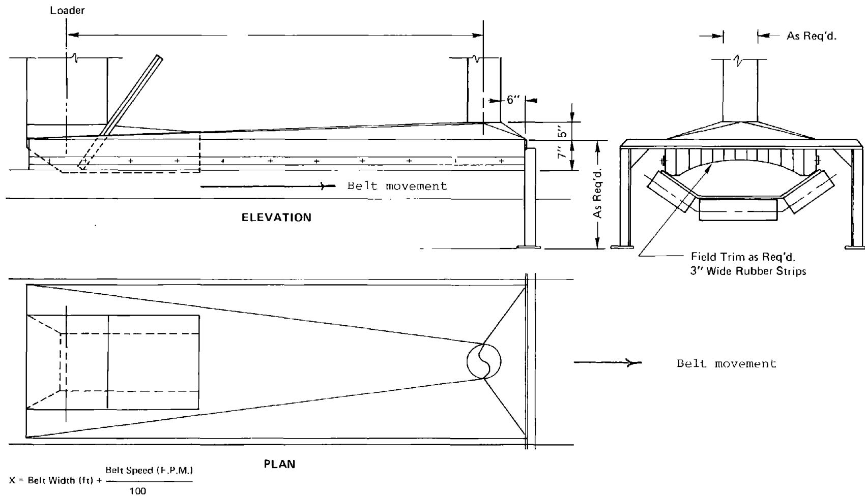
FIGURE 3-3 Loader hood.
