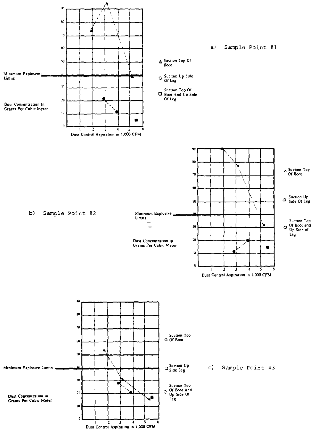
FIGURE C-3 Dust concentrations at three sample points.
