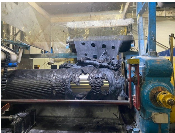
Figure A2. Breakdown mill number 1. Photo by NIOSH.
