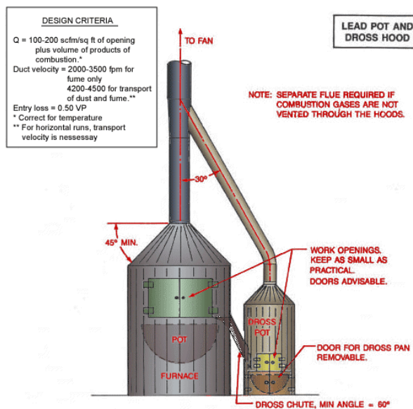
Figure B13. Enclosed lead pot and dross hood [OSHA 2024].
