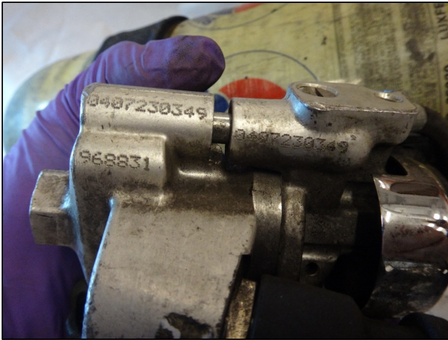
Figure 17: Cylinder attachment overview with bell assembly and markings
