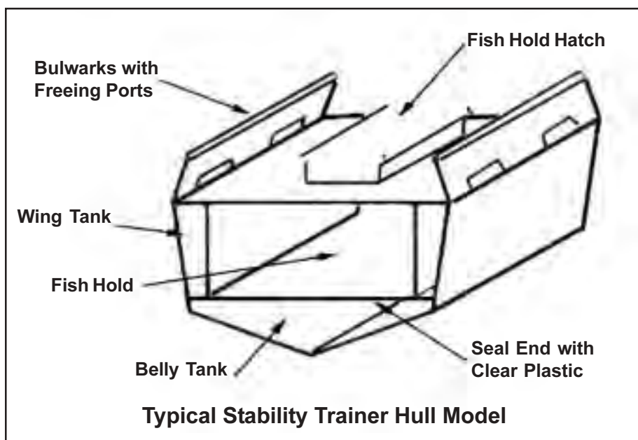
Figure 1: Base model section shown. Additional features such as fish hold pen boards, tank and void vents, outriggers with paravanes, and net reels will be added to individual sets of models to illustrate specific stability characteristics.
