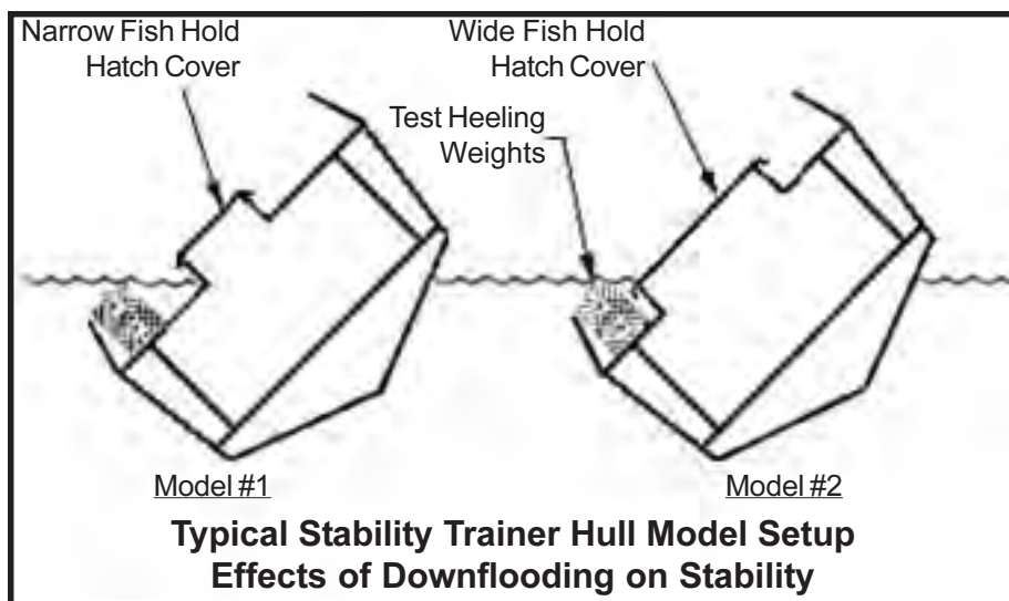
Figure 3: Set of two models are used to illustrate the effect of downflooding from fish hold hatches on stability. Test heeling weights are added one at a time to demonstrate the model’s relative level of stability. The training model with the stability effect, in this case model 2, will capsize well before the other one.
