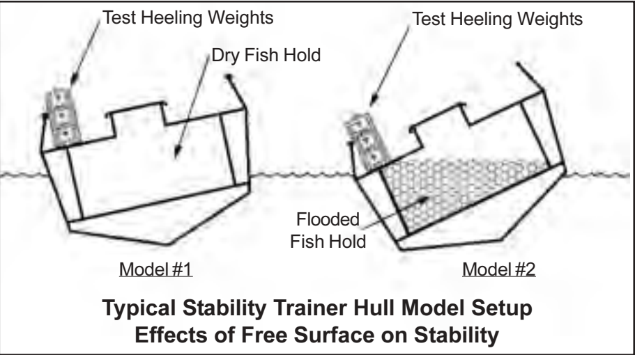
Figure 2: A set of two models are used to illustrate the effect of free surface from partially flooded fish hold on stability. Test heeling weights are added one at a time to show each model’s relative level of stability. The training model with the stability defect, in this example model 2, will capsize well before the other model.
