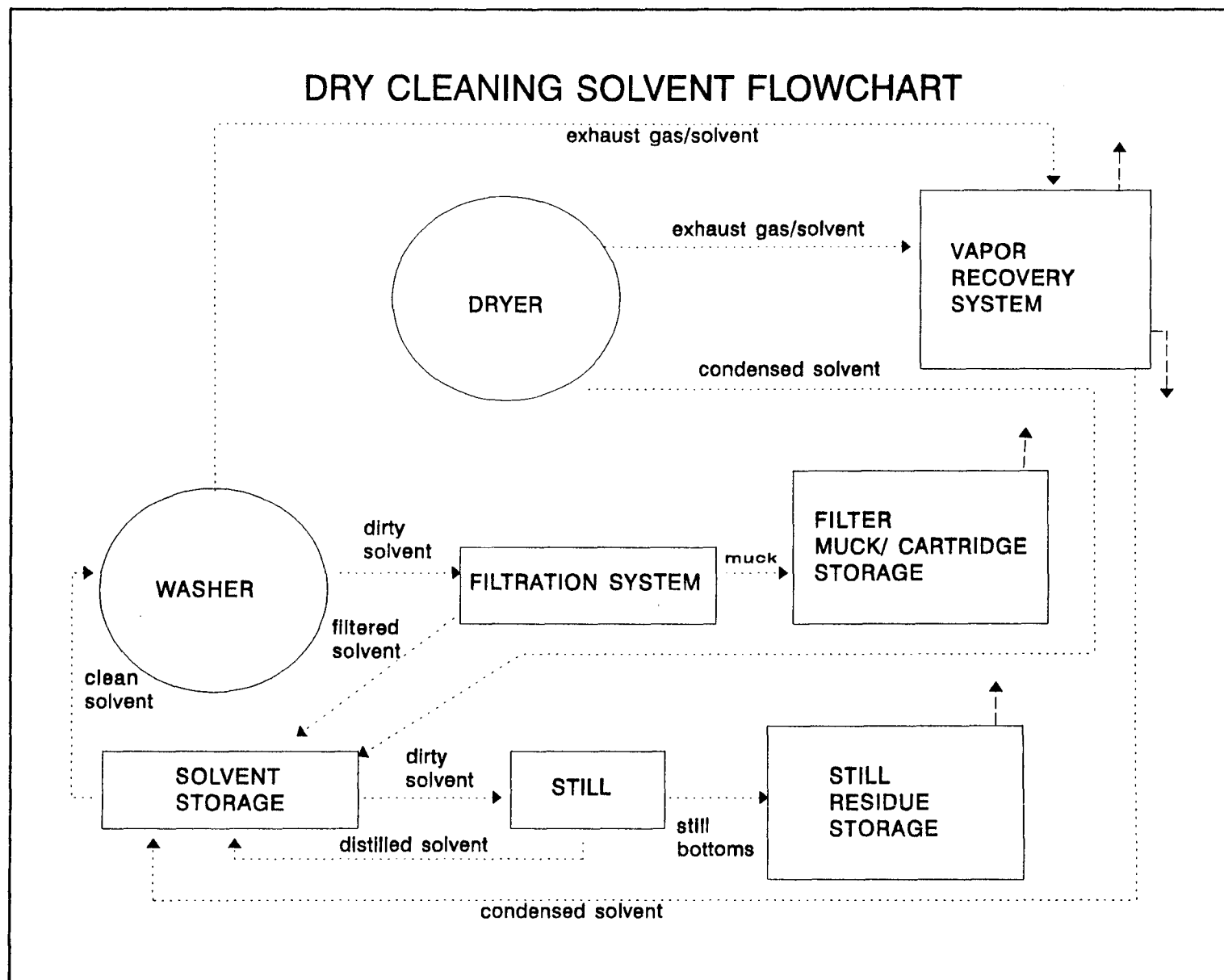
Figure 2. Solvent Flow Chart.
