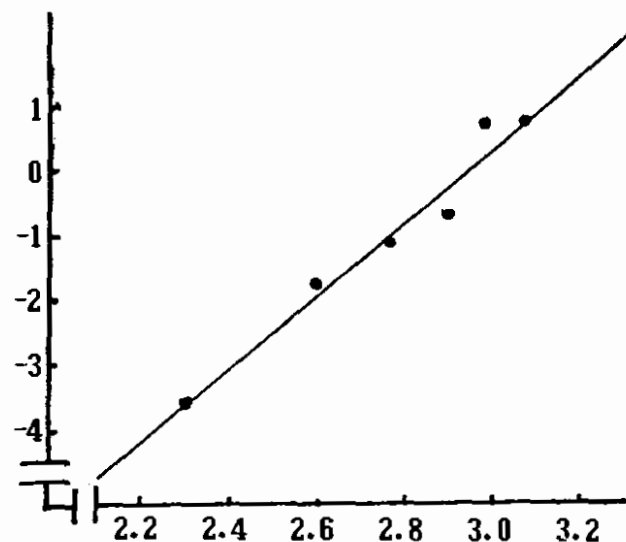
Figure 1. The correlation between logarithmic doses and logit.
