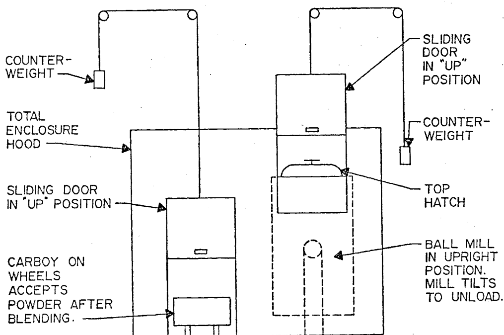
Figure 4-2. Front view of typical ball mill and hood enclosure.
