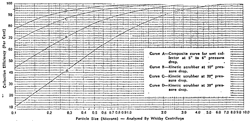
Figure 3-8. Published efficiency curve for wet collector (13).
