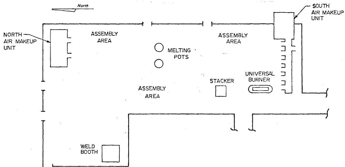
Figure 1-1. View of worker station and collection system.
