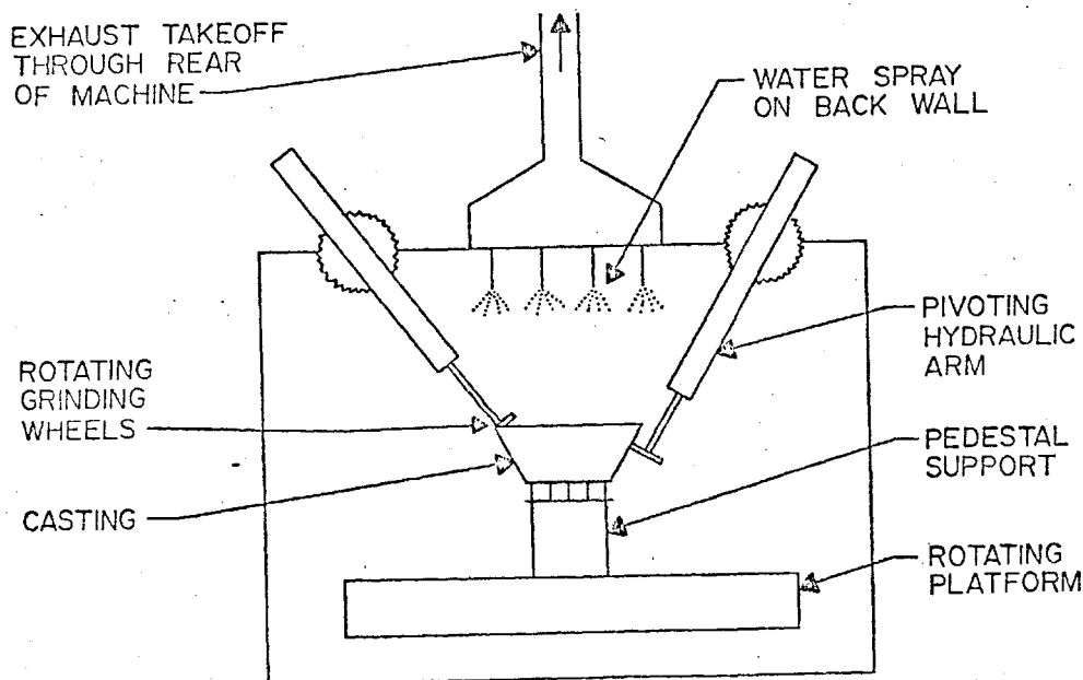
Figure 3-2. Front view of grinding machine showing details of process and hood.
