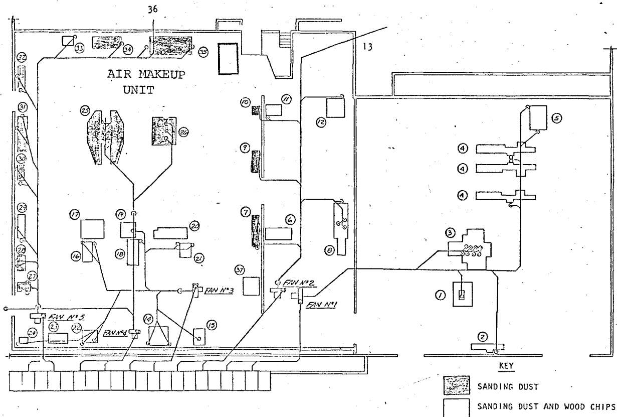
Figure 2-1. Plant layout.
