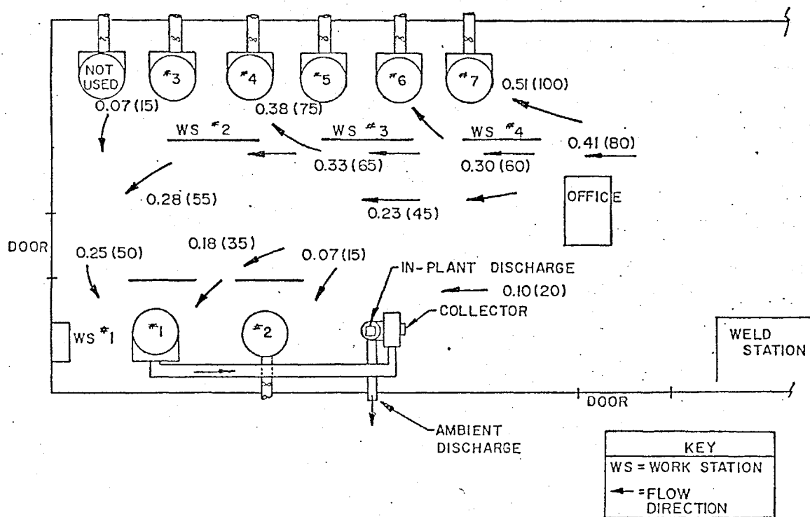
Figure 3-6. Air velocity patterns, m/sec (ft/min).
