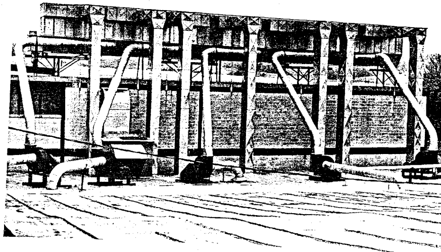
Front view of inlet ducts, fans, collector modules, and outlet ducts. Woodworking room is located below roof in foreground.
