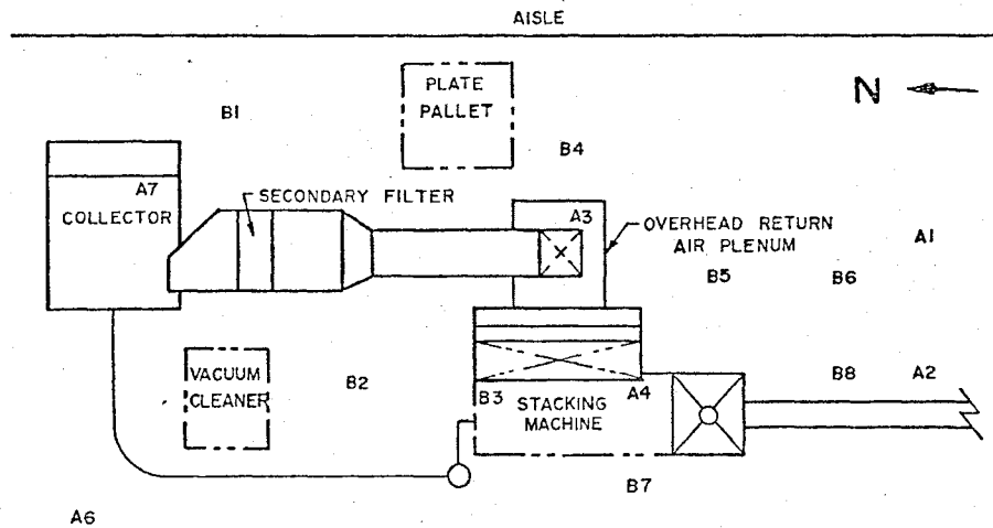
Figure 1-3. Area sampling locations.
