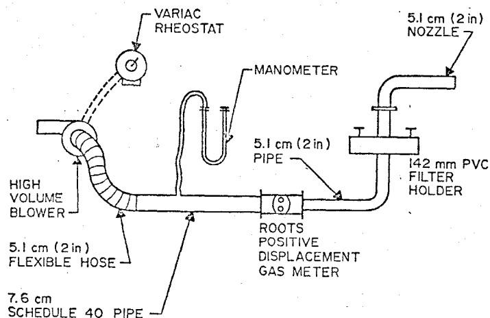
Figure 3. High volume sampling train.
