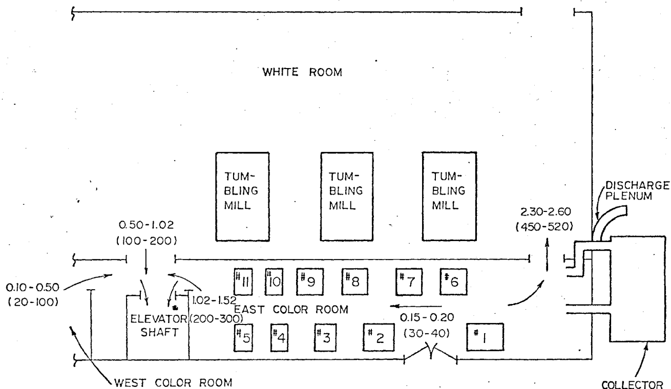
Figure 4-4. Air velocity patterns after recirculation, m/sec (ft/min).
