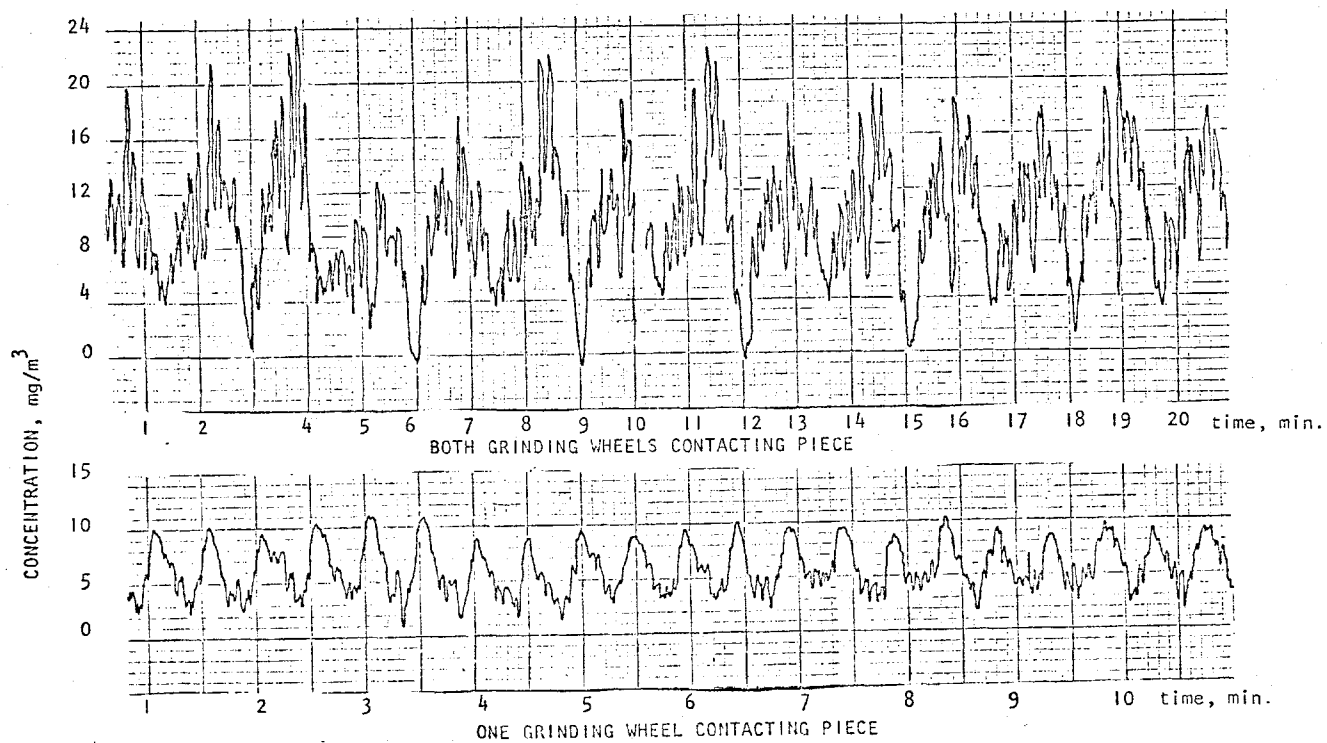
Figure 3-7. Typical outlet concentration plots.
