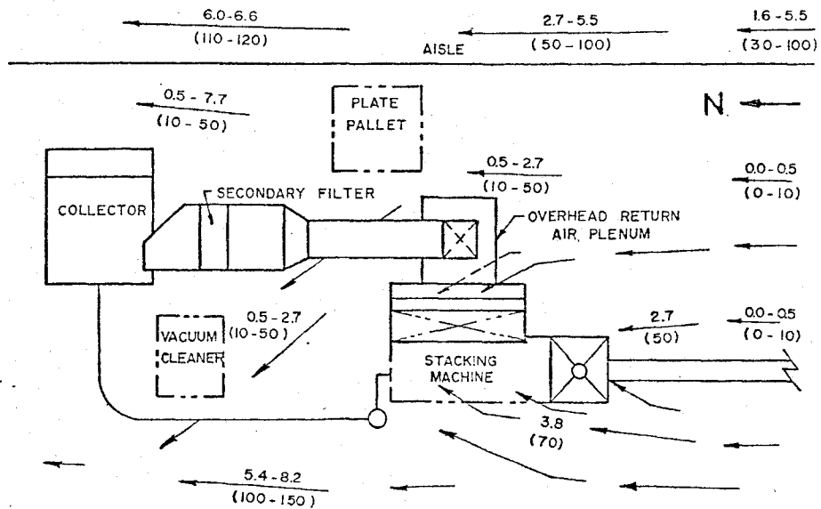
Figure 1-3. Area sampling locations.
