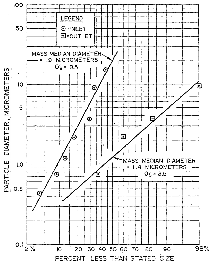
Figure 3-4. Particle size distribution plots.
