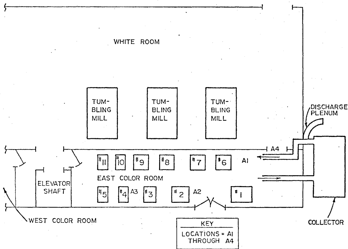
Figure 4-3. Area sampling locations.
