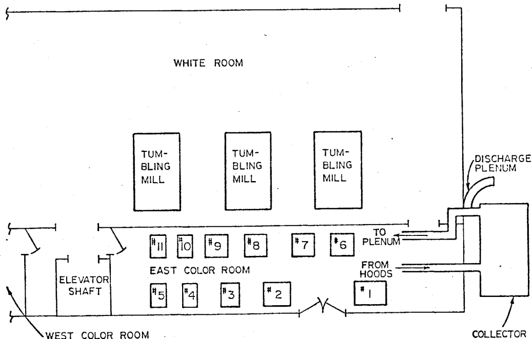
Figure 4-1. Plant layout.
