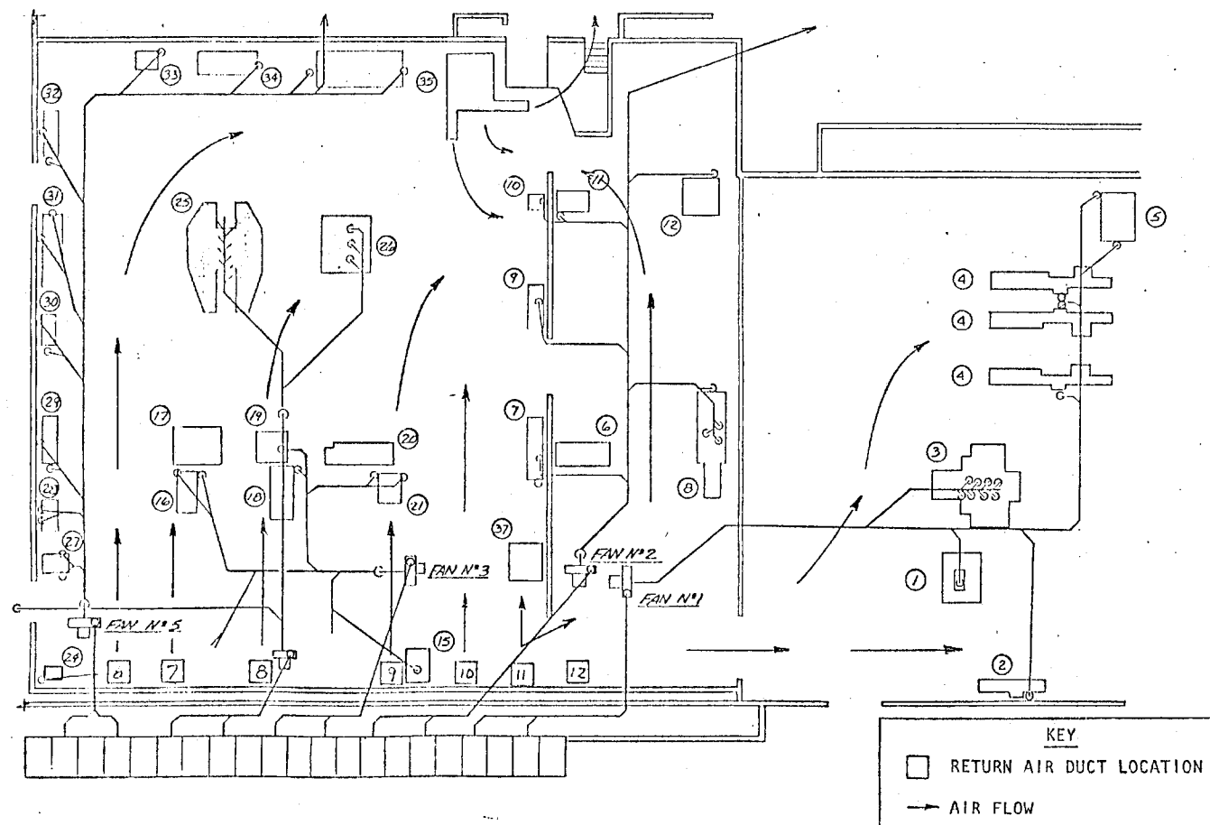
Figure 2-5. Air velocity patterns in machine rooms.
