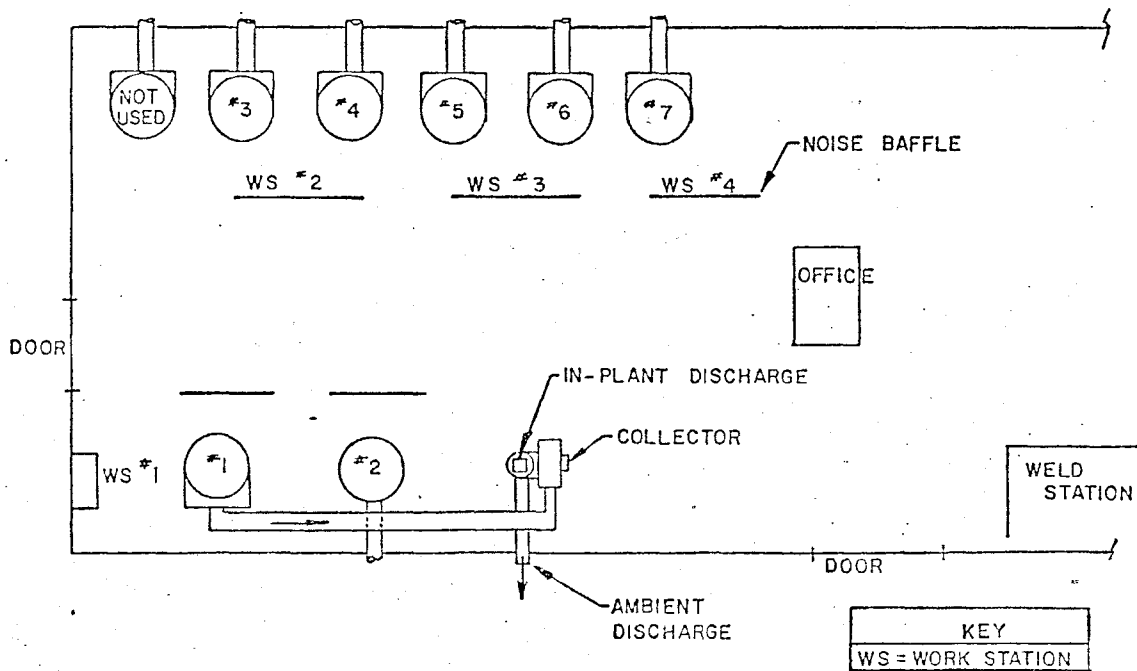
Figure 3-1. Layout of grinding area at one end of high bay area.
