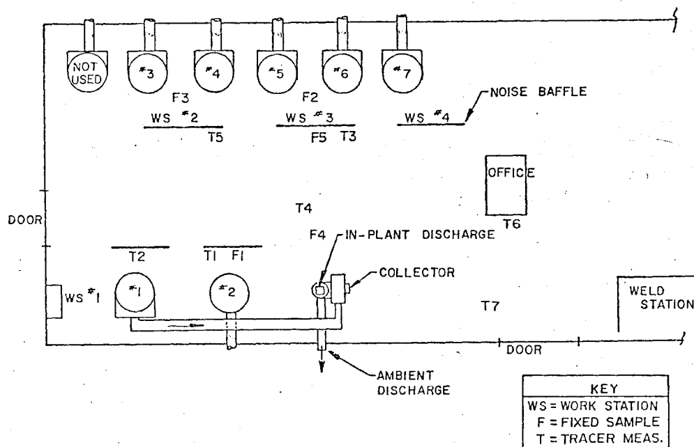
Figure 3-5. Area sampling locations.
