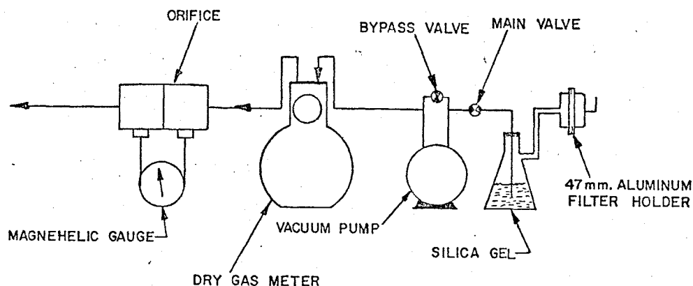
Figure 2. In-stack sampling train.
