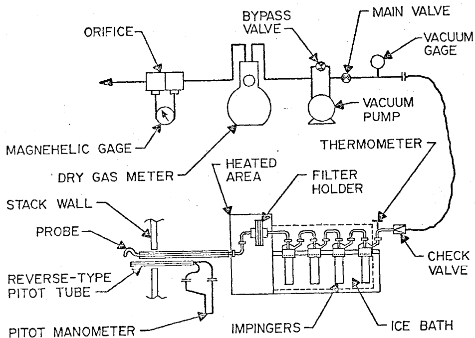
Figure 1. EPA method 5 sampling train.
