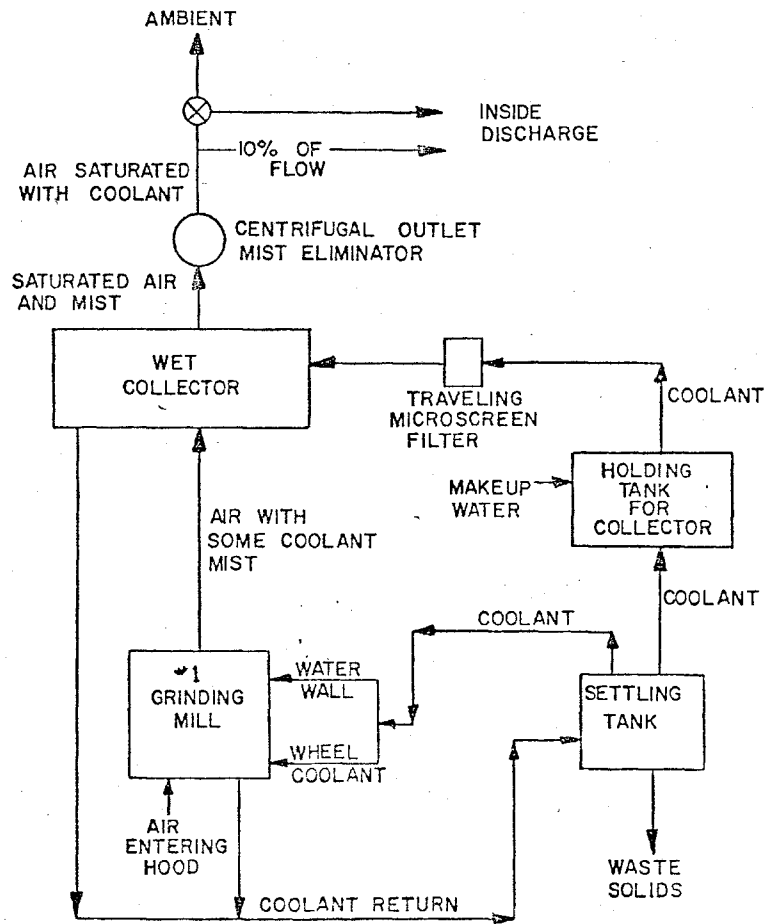
Figure 3-3. Air and coolant cycle.
