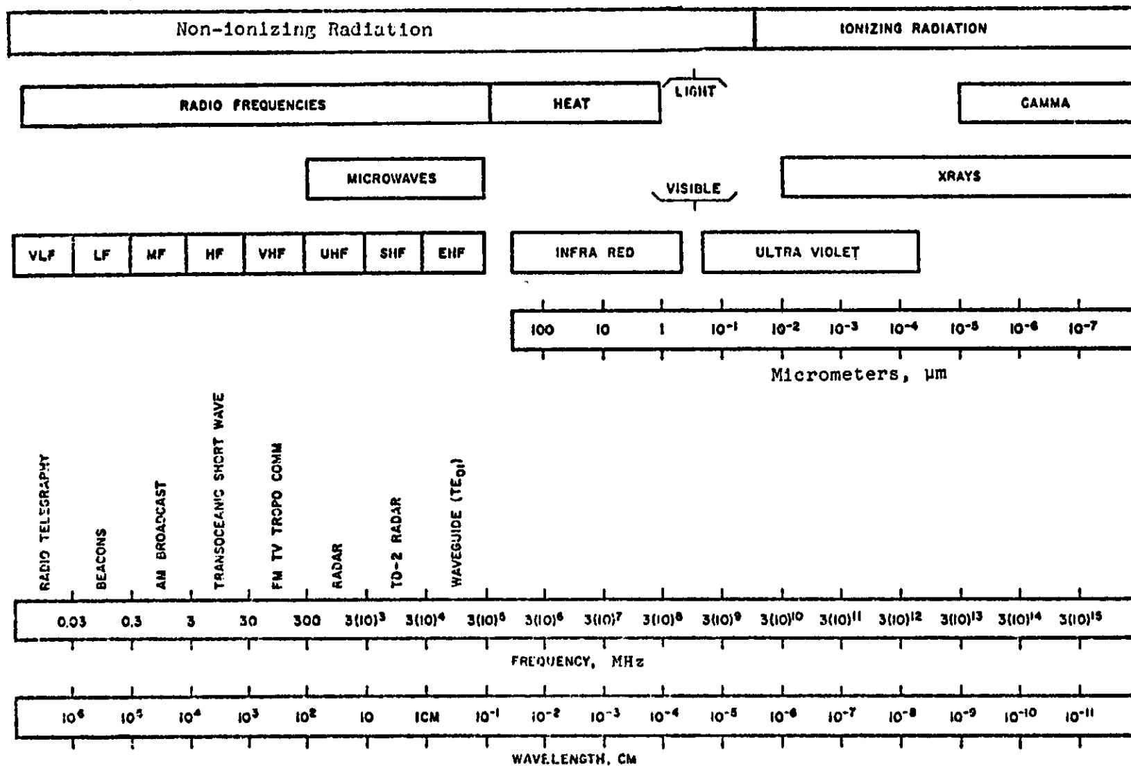
Mumford WW: Some Technical Aspects of Microwave Radiation Hazards. Proc. IRE 49:427-47, 1961. Figure 28-1. The Electromagnetic Spectrum.
