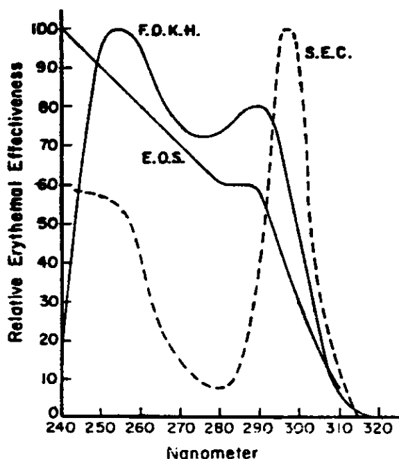
Figure 28-2. Comparison of Standard Erythematous Curve (S.E.C.) with Relative Erythematous Effectiveness Curves of Everett, Olsen and Soyer (E.O.S.) and Freeman, Owens, Knox and Hudson (F.O.K.H.).
