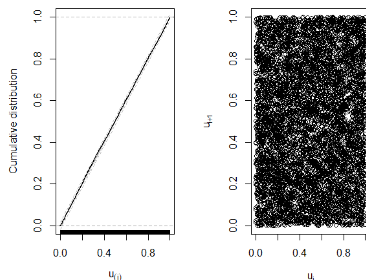
E. Twinstim model: 250 meters, 7 days
