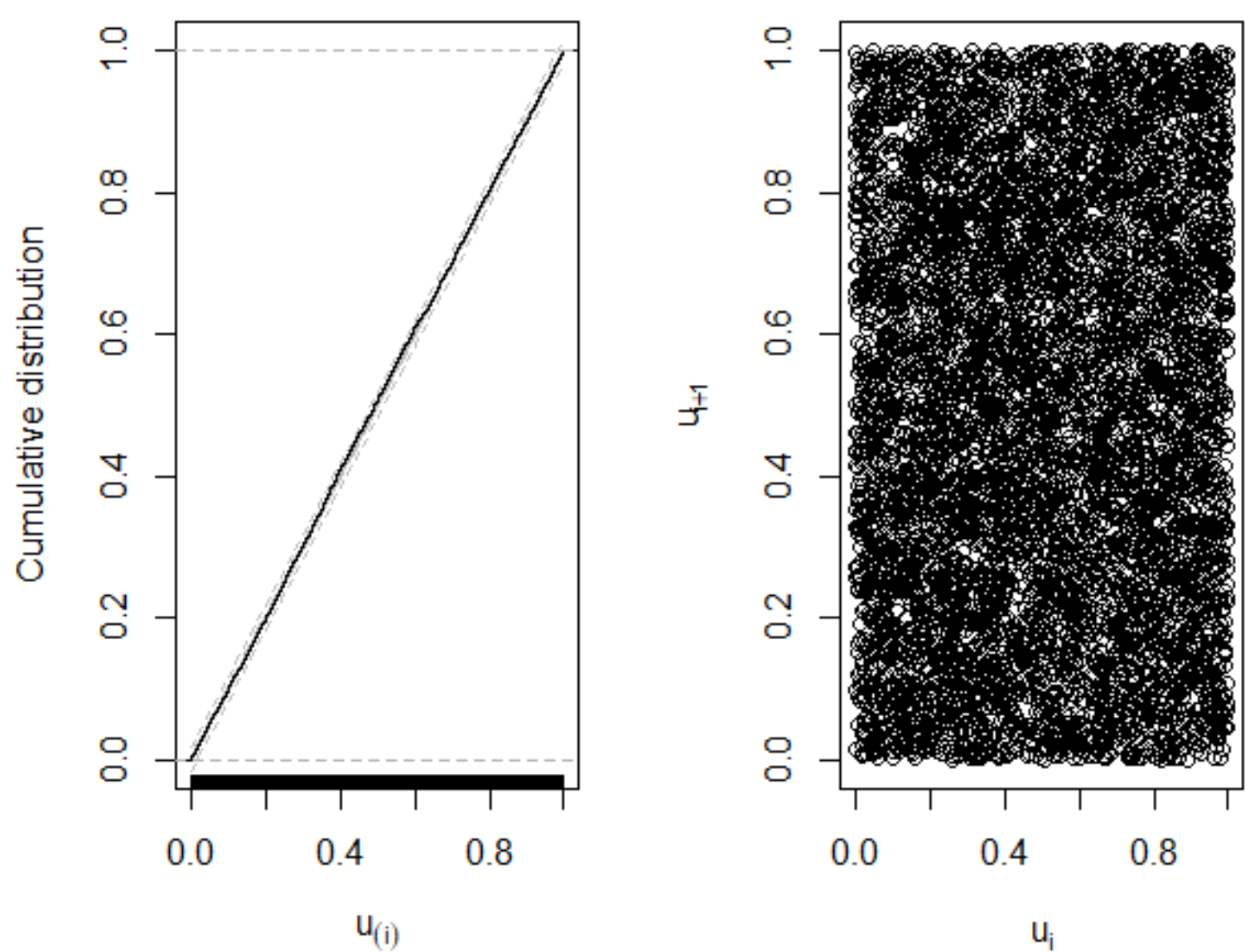
B. Twinstim model: 100 meters, 7 days
