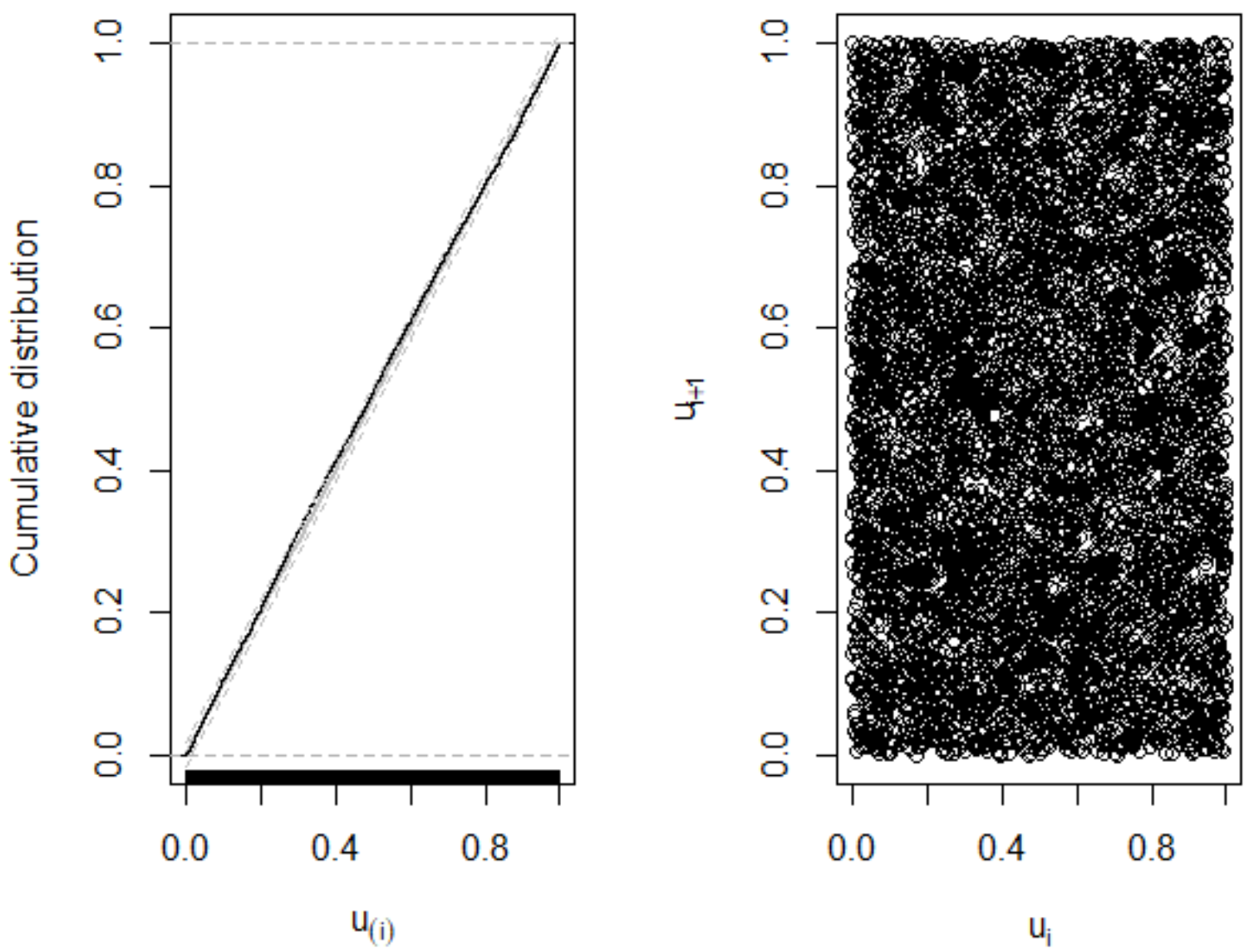
C. Twinstim model: 100 meters, 14 days
