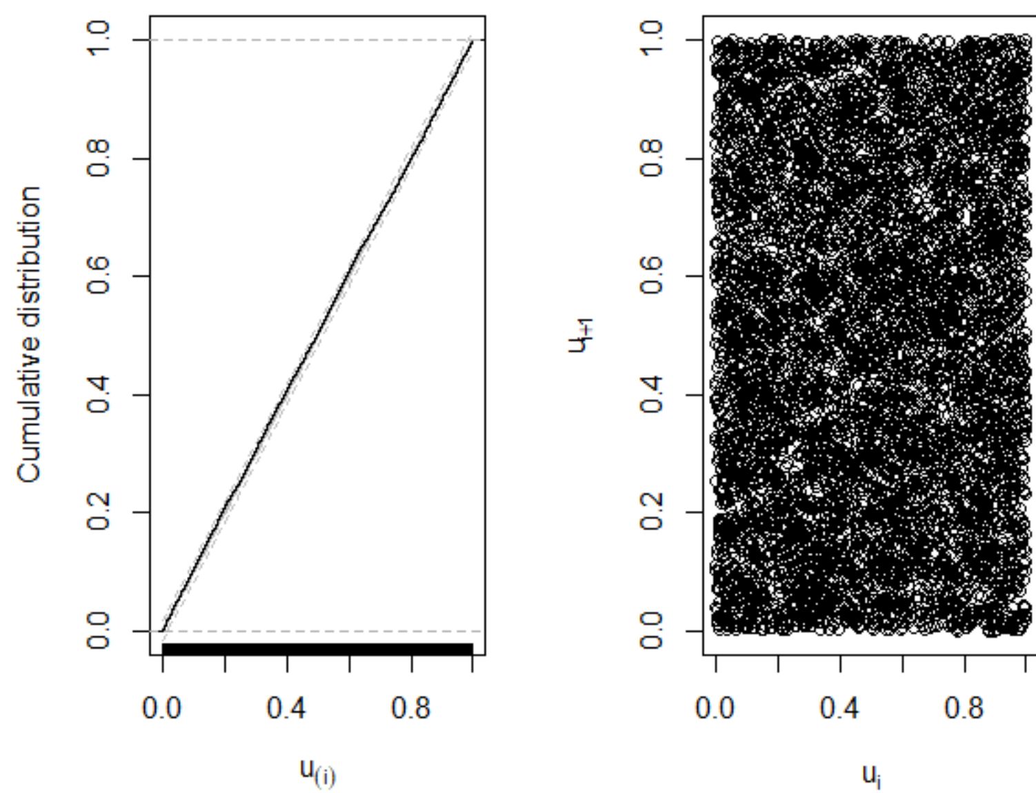
D. Twinstim model: 250 meters, 3 days
