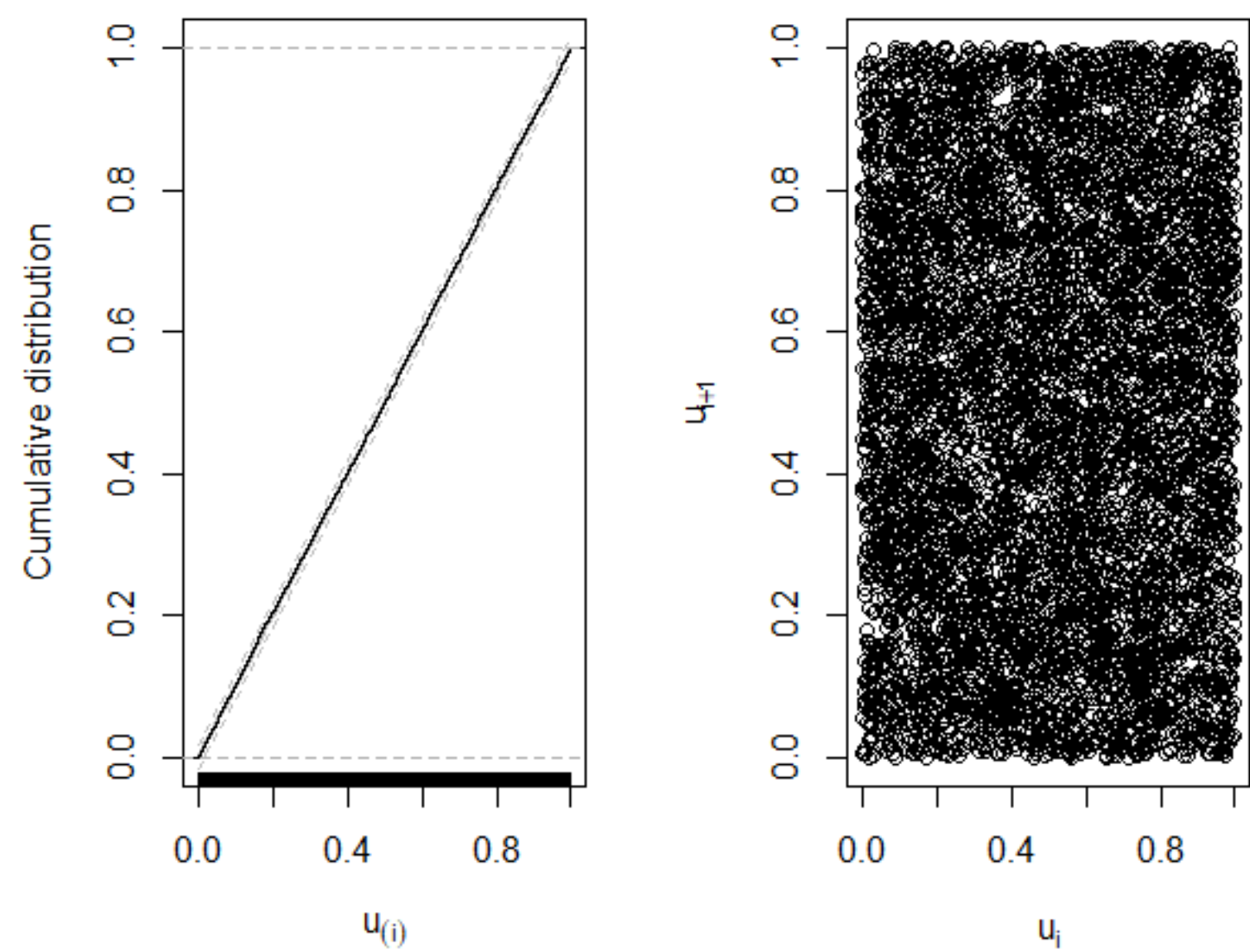
A. Twinstim model: 100 meters, 3 days
