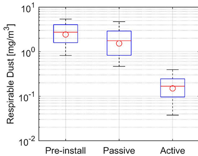
Fig. 9. Respirable dust concentrations. On each box, the central mark indicates the median, and the bottom and top edges of the box indicate the 25th and 75th percentiles, respectively. The whiskers extend to the most extreme data points
