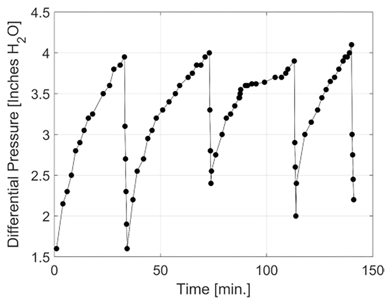
Fig. 5. Typical changes in differential pressure during testing
