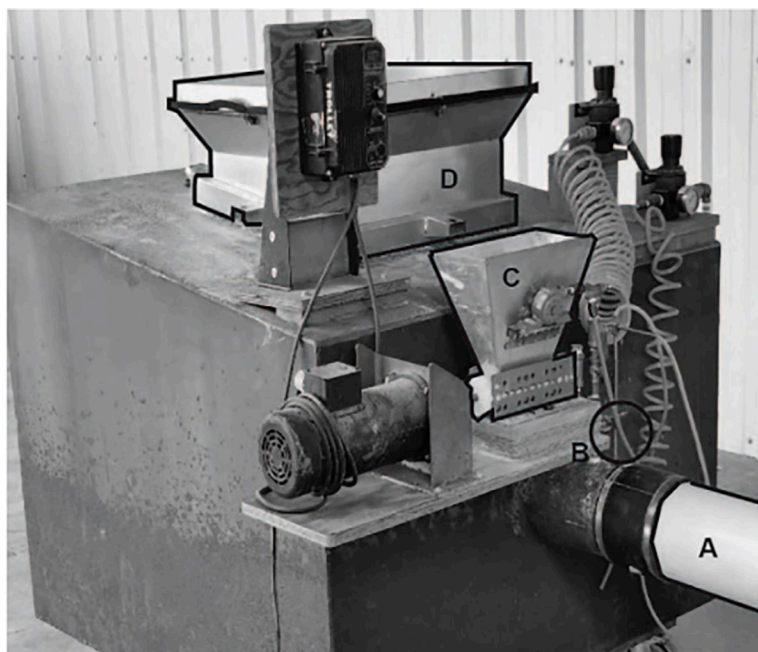
Fig. 4. Experimental setup for dust collector tests: (A) air inlet, (B) ports for flow measurement and dust injection, (C) dust generator, and (D) flange for mounting the Dustinator
