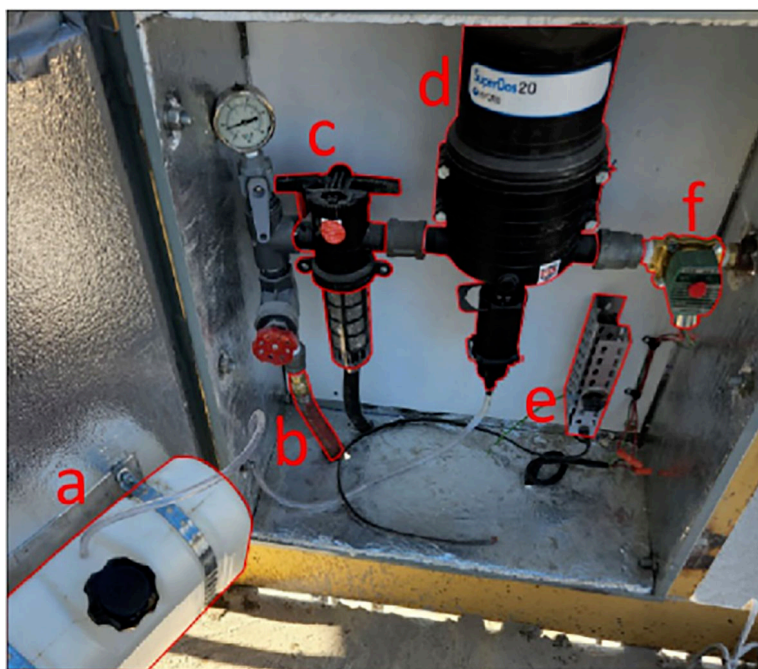
Fig. 3. Benetech®'s prototype dust suppression system, enclosed in an insulated cabinet for installation at the CPM site: (a) surfactant tank, (b) 80-psi water inlet, (c) back-flushable filter, (d) surfactant pump, (e) heater, and (f) solenoid valve
