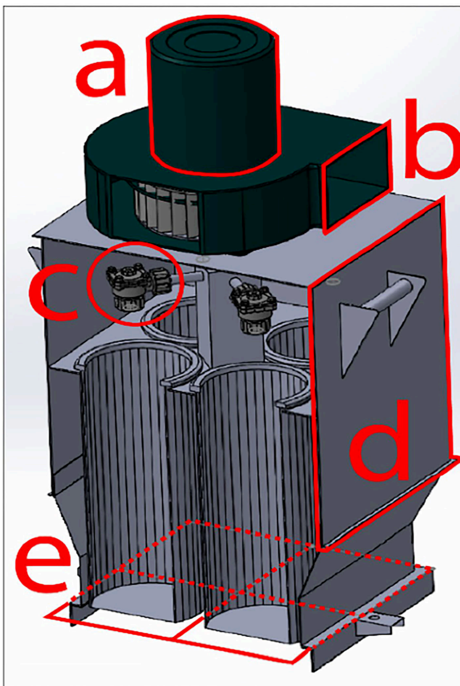
Fig. 2. Prototype filtration system (“Dustinator”) tested by NIOSH: (a) powered blower (220v-3HP), (b) clean air exit, (c) jet pulse nozzles (4 each), (d) filter housing, and (e) mounting flange and dust/air inlet
