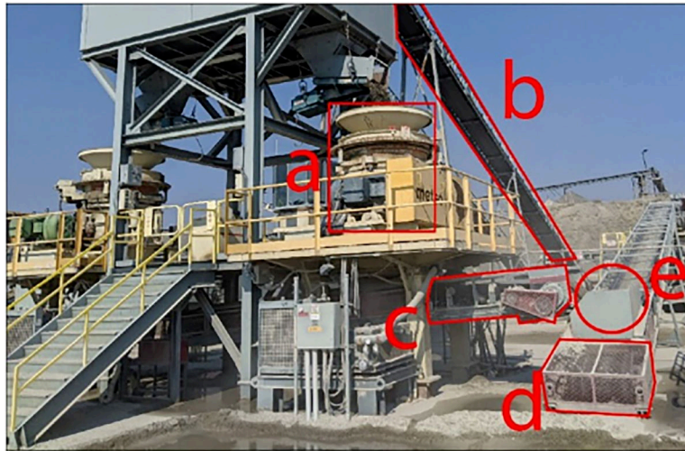
Fig. 6. Crusher/conveyor system at the CPM site, before installation of the dust control system: (a) crusher #2, (b) feed conveyor #2, (c) head end of horizontal conveyor #15, (d) tail end of return conveyor #13, and (e) transfer point
