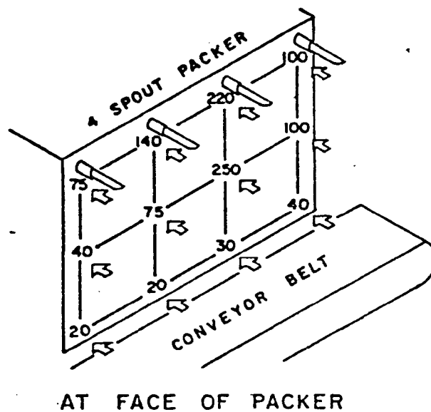
Figure H: Ventilation at Main Product Packing Area
