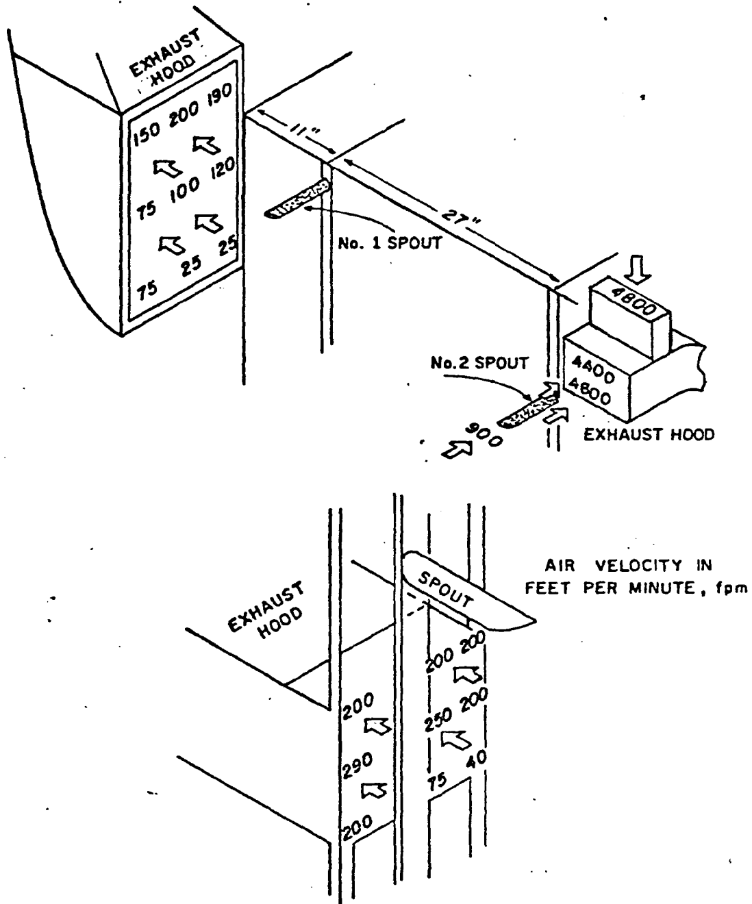
Figure K: Ventilation at Fine Product Packing Areas
