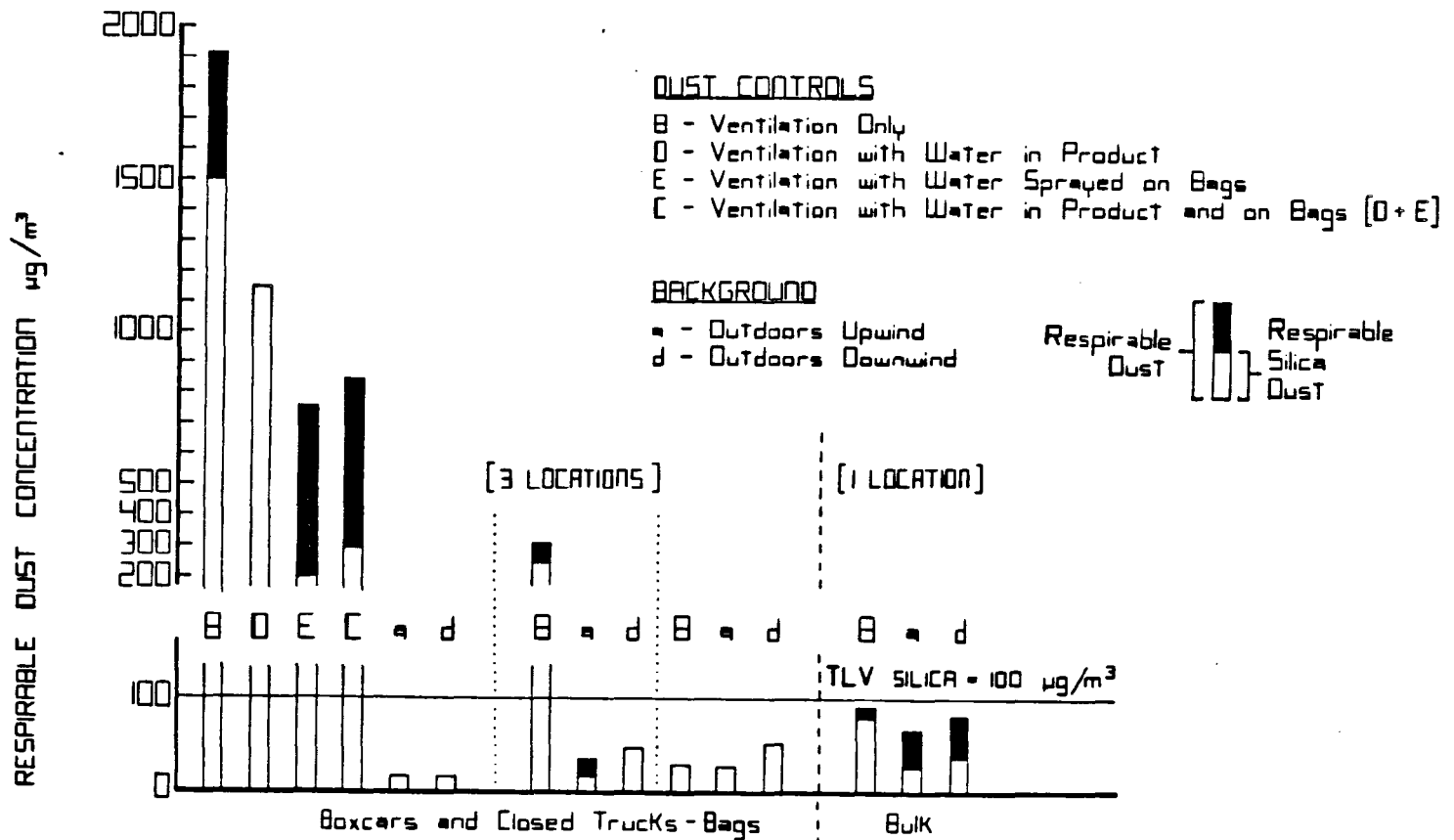
Figure D: DUST CONCENTRATION AT LOADING
