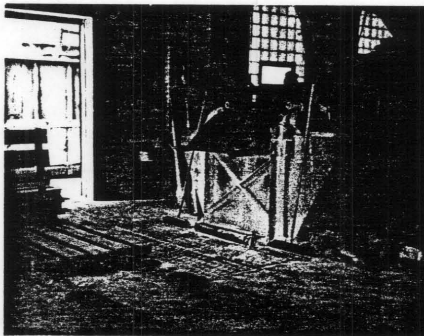
7. Down draft floor grill; dry sweeping of spills; broken bags at dust source
