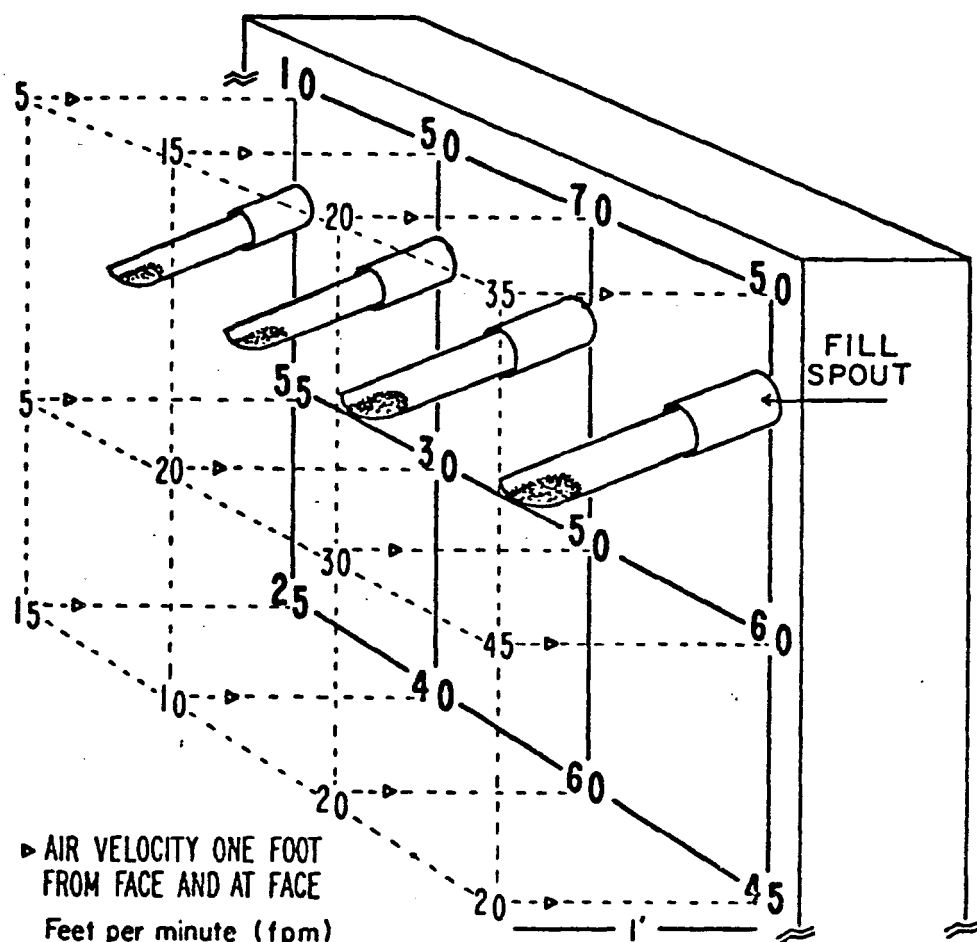
Figure F: Ventilation measurements - Main Product Packer
