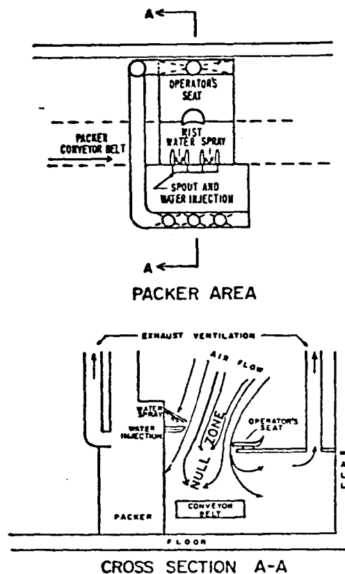
Figure E: Packer - Ventilation and Water Controls
