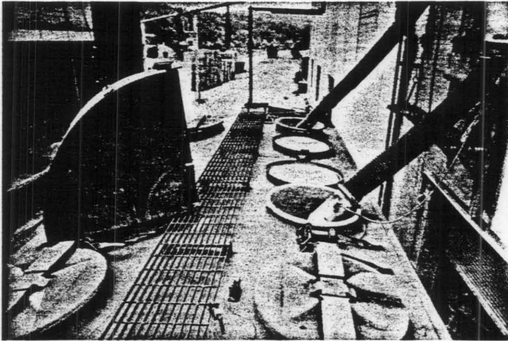
13. Bulk loading closed railroad hopper car with exhaust; fill-spouts and exhaust
