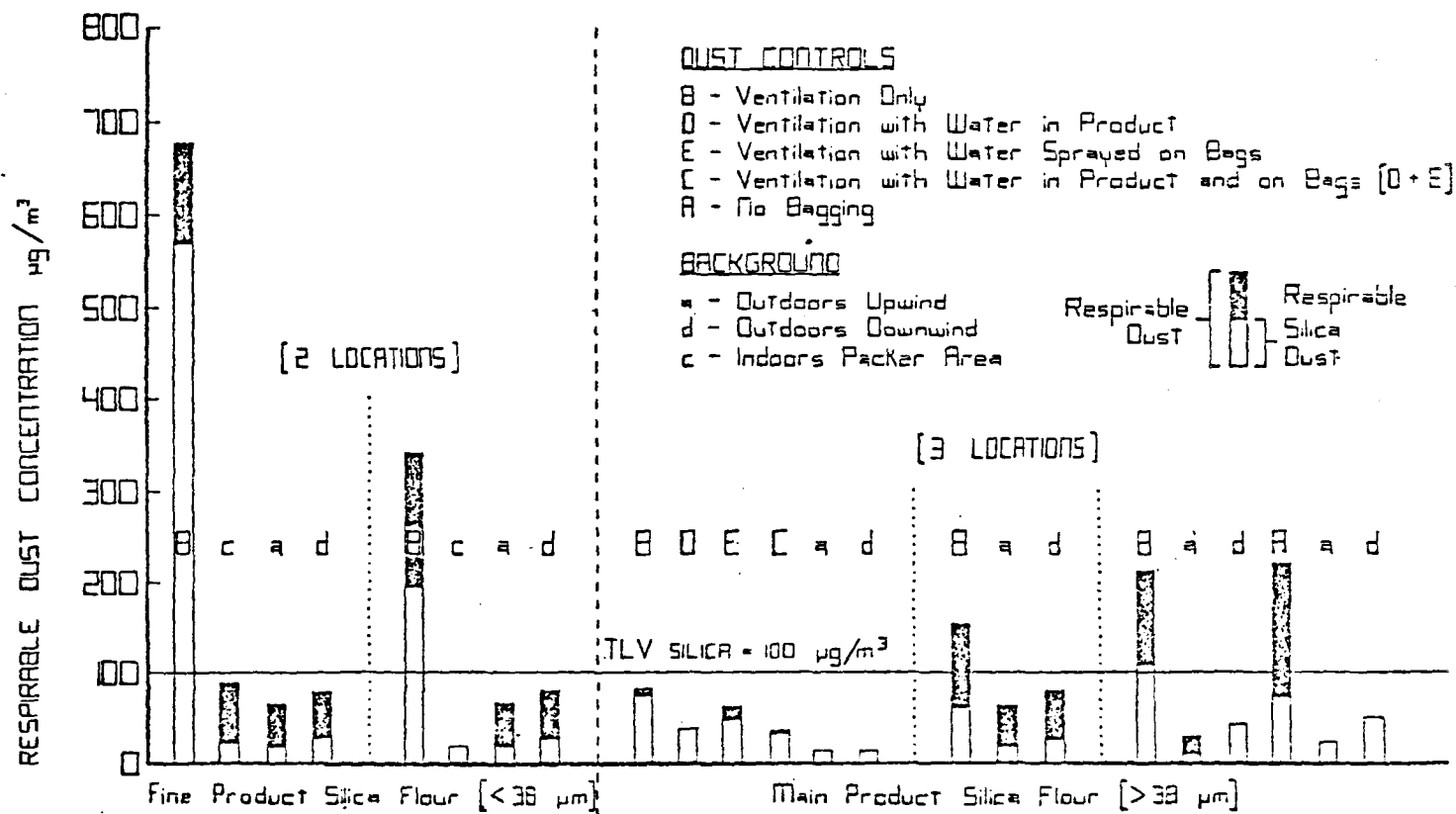
Figure B: DUST CONCENTRATION AT PACKERS
