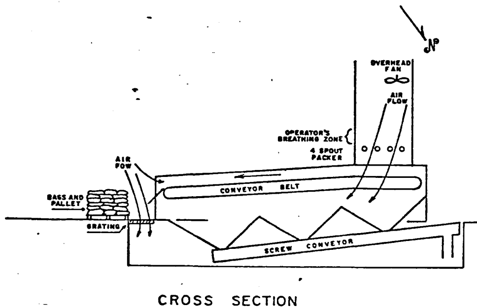
Figure G: Packing Area - Main Product
