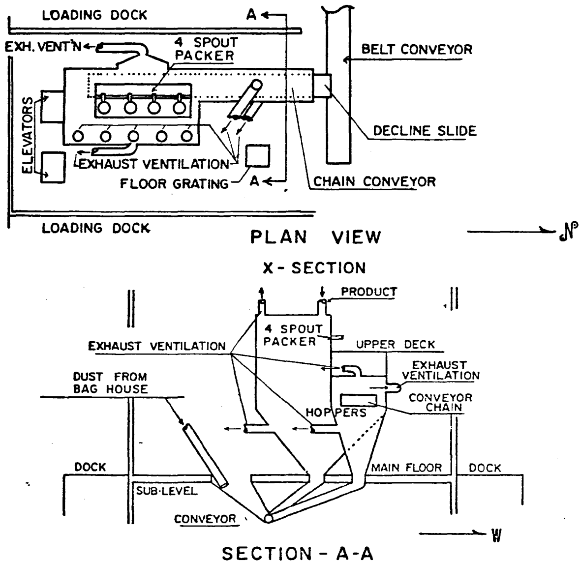
Figure I: Packing Area - Main Product
