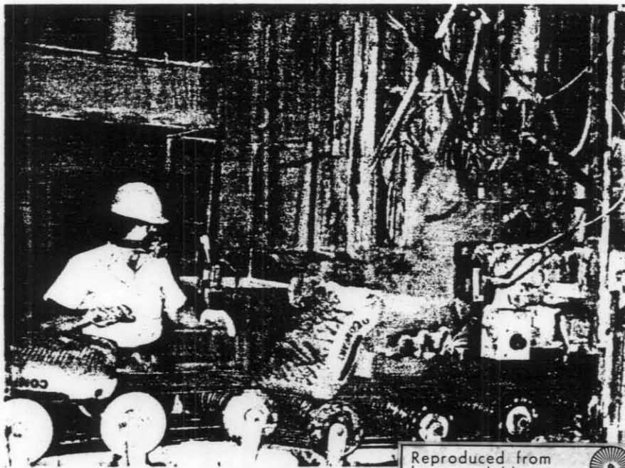
5. Conveyor transfer point excessive bag drop, broken bag, incomplete spray capture, use of respirator
