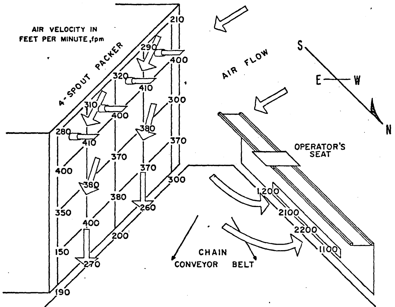
Figure J: Ventilation at Main Product Packing Area
