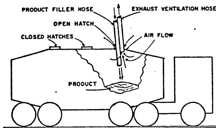
CLOSED HOPPER TRUCK (FLOUR) LOADING
