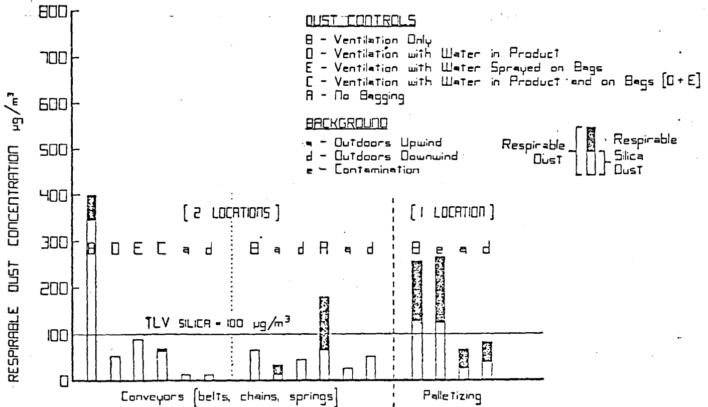
Figure C: DUST CONCENTRATION FOR BAG HANDLING
