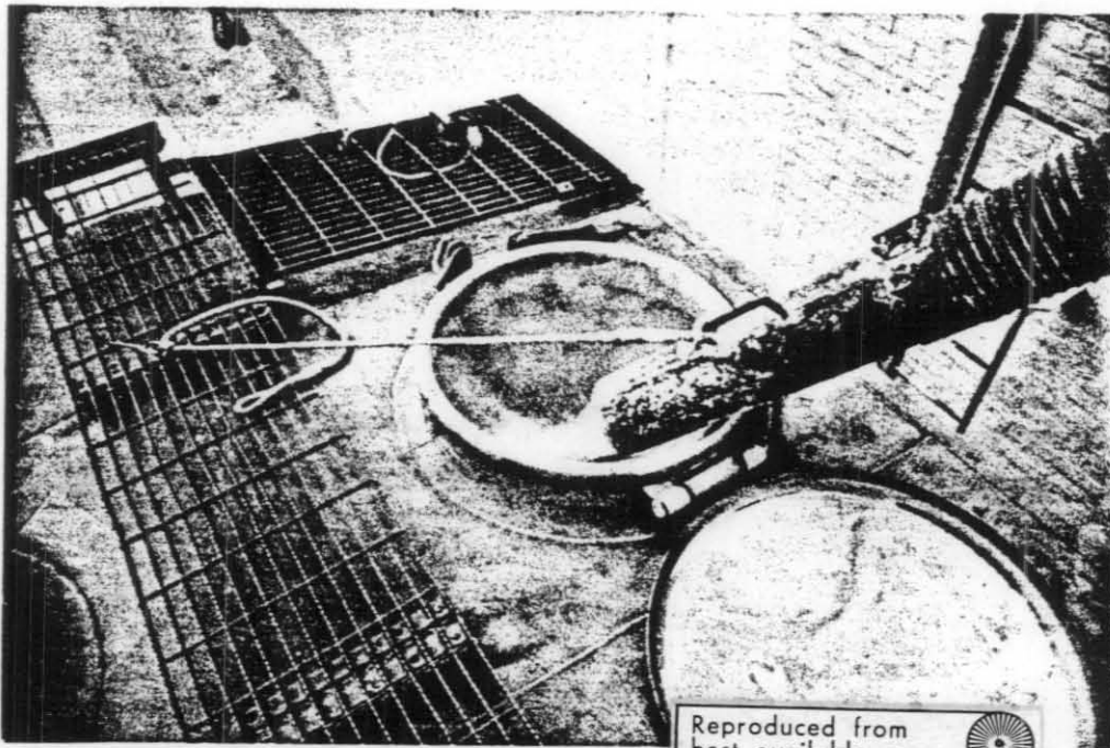
14. Bulk loading closed railroad hopper car with exhaust
