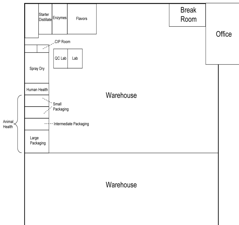
Figure 1. Plant layout
