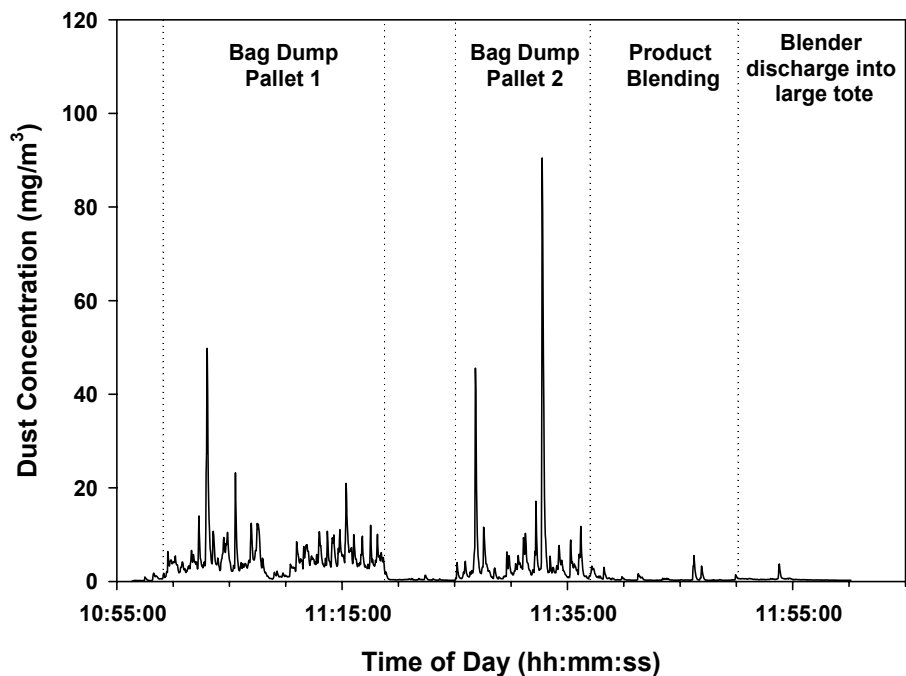
Figure 10. Real-time measurements of dust exposure for a worker in the large packaging room during bag dumping, blending, and blender discharge activities, December 4, 2007
