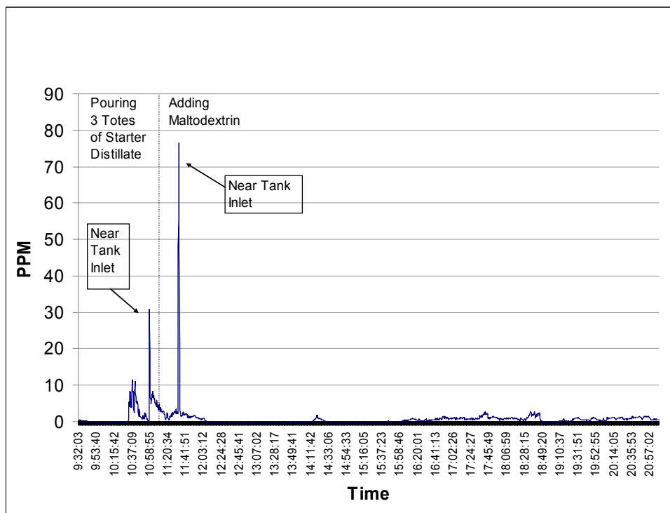
Figure 6. Real-time measurements of diacetyl air concentrations measured by FTIR in the spray dry room on December 3, 2007 during the production of butter flavored powder using starter distillate (50X)
