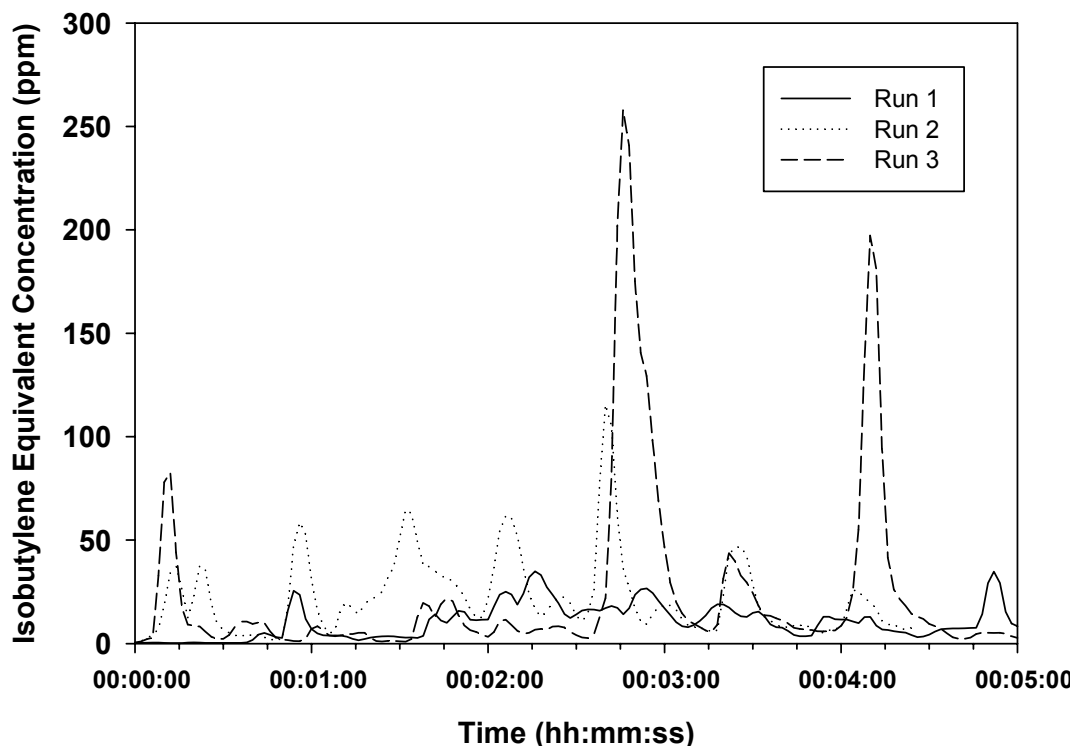
Figure 3. Real-time measurements of personal VOC concentrations for a worker in the starter distillate room during the manual transfer of the starter distillate (three transferring operations are overlaid on one graph), December 3, 2007
