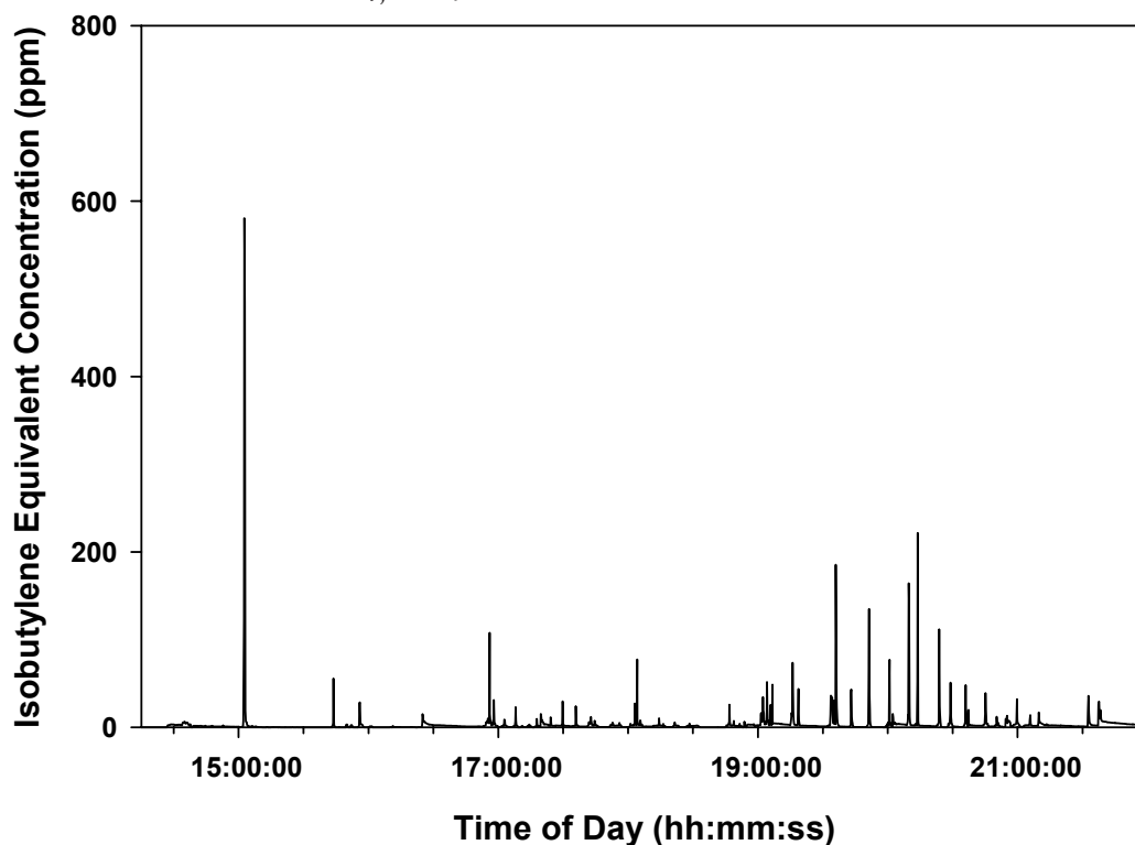
Figure 5. Real-time measurements of personal VOC concentrations for a worker in the spray dry room during slurry preparation and packaging activities for Natural Butter 50X, December 4, 2007
