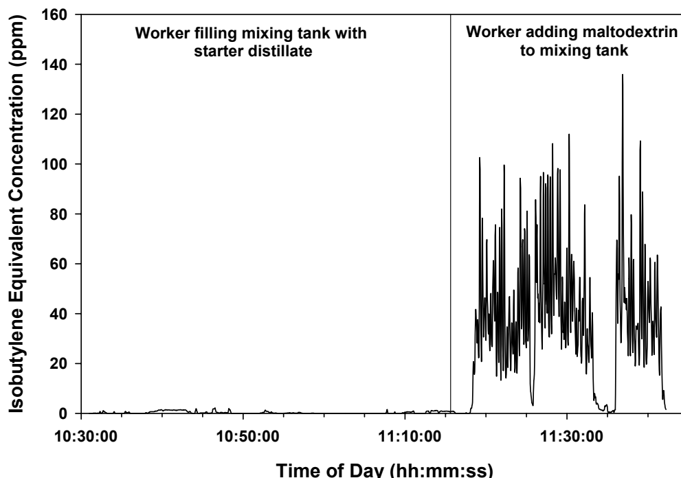
Figure 4. Real-time measurements of personal VOC concentrations for a worker in the spray dry room during the preparation of the slurry feed for ESD-50X, December 3, 2007
