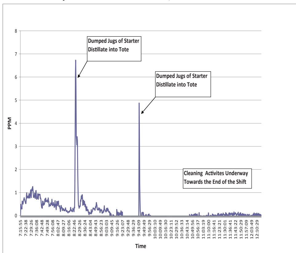
Figure 8. Real-time measurements of diacetyl air concentrations measured by FTIR in the starter distillate room during starter distillate production on December 5, 2007
