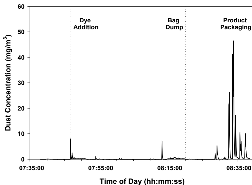
Figure 11. Real-time measurements of dust exposure for a worker in the intermediate packaging room during dye addition, bag dumping, and product packaging activities for BioPlus®, December 5, 2007
