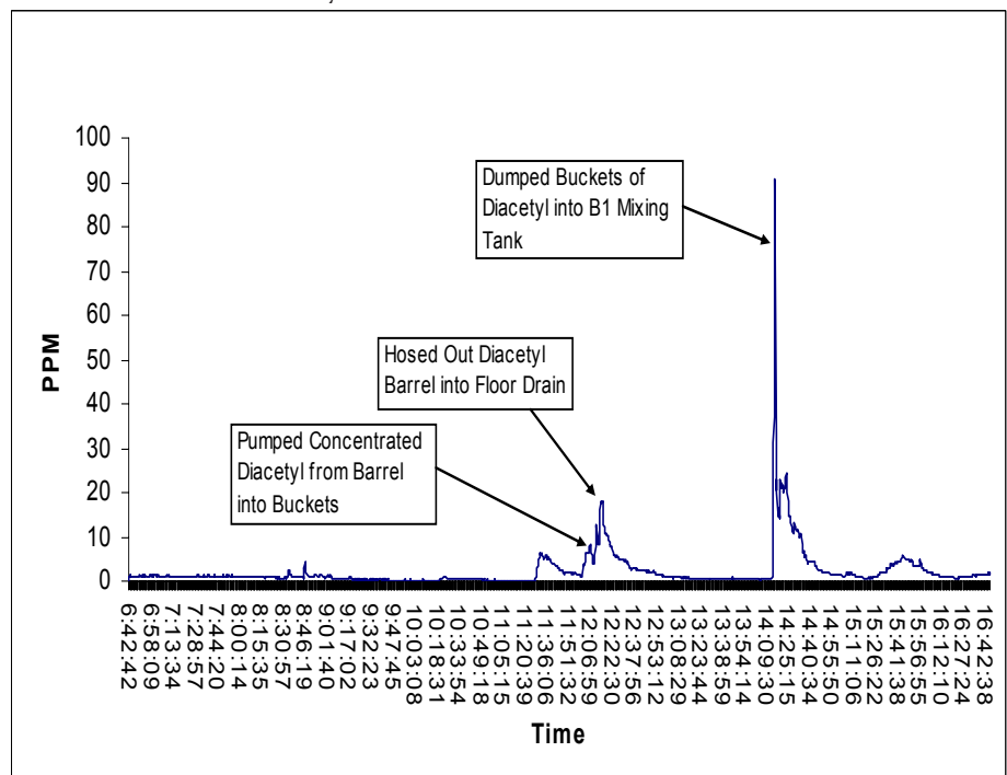
Figure 7. Real-time measurements of diacetyl air concentrations measured by FTIR in the spray dry area on December 4, 2007 during the production of a butter flavored powder using concentrated diacetyl
