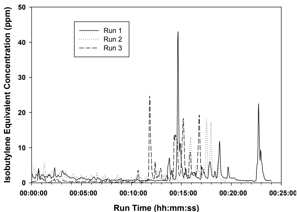
Figure 2. Real-time measurements of personal VOC concentrations for a worker in the starter distillate room during filling of the stills with fermented milk stock (three operations of filling the stills are overlaid on one graph), December 3, 2007
