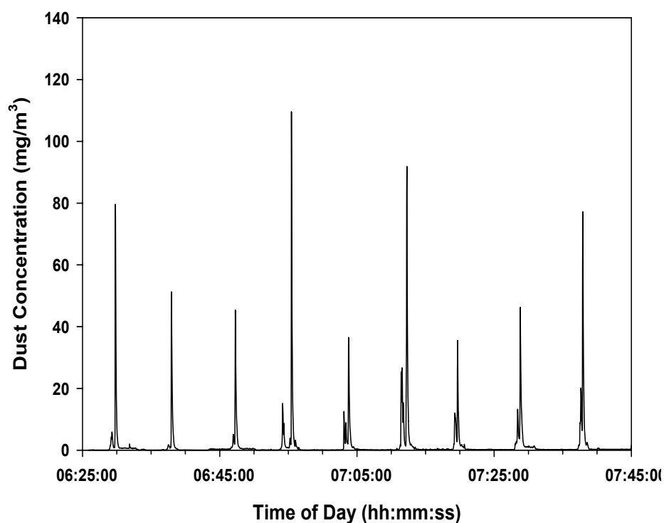
Figure 9. Real-time measurements of dust exposure for a worker in the spray dry room during the packaging of ESD-50X, December 4, 2007
