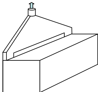
Figure 4. Example of a slot ventilation hood for the screen printing table.
