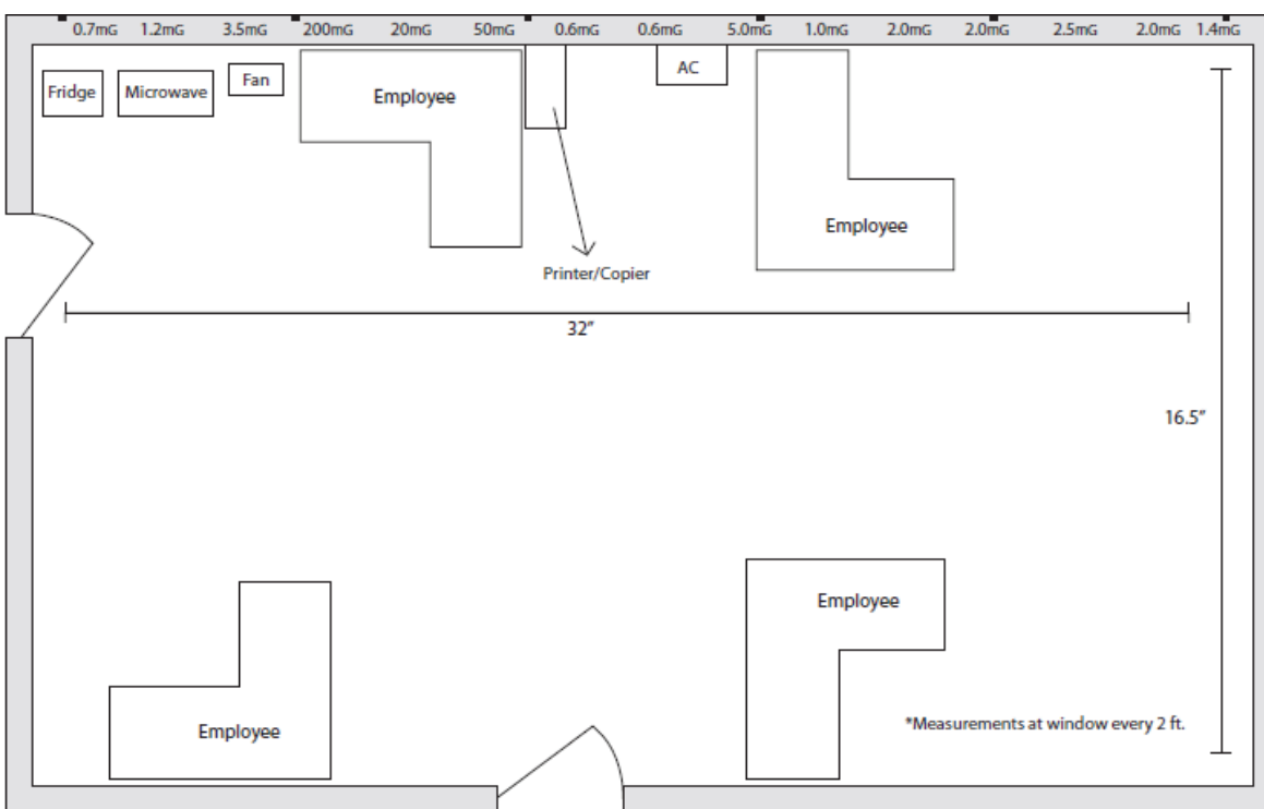
Figure 2. Scale layout of the timekeeping office showing magnetic field measures along the interior wall nearest the transformer.
