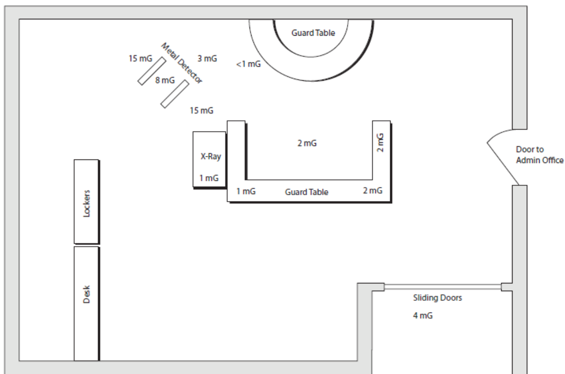
Figure 4. Magnetic field measurements in front lobby of the Lebanon Correctional Institution.
