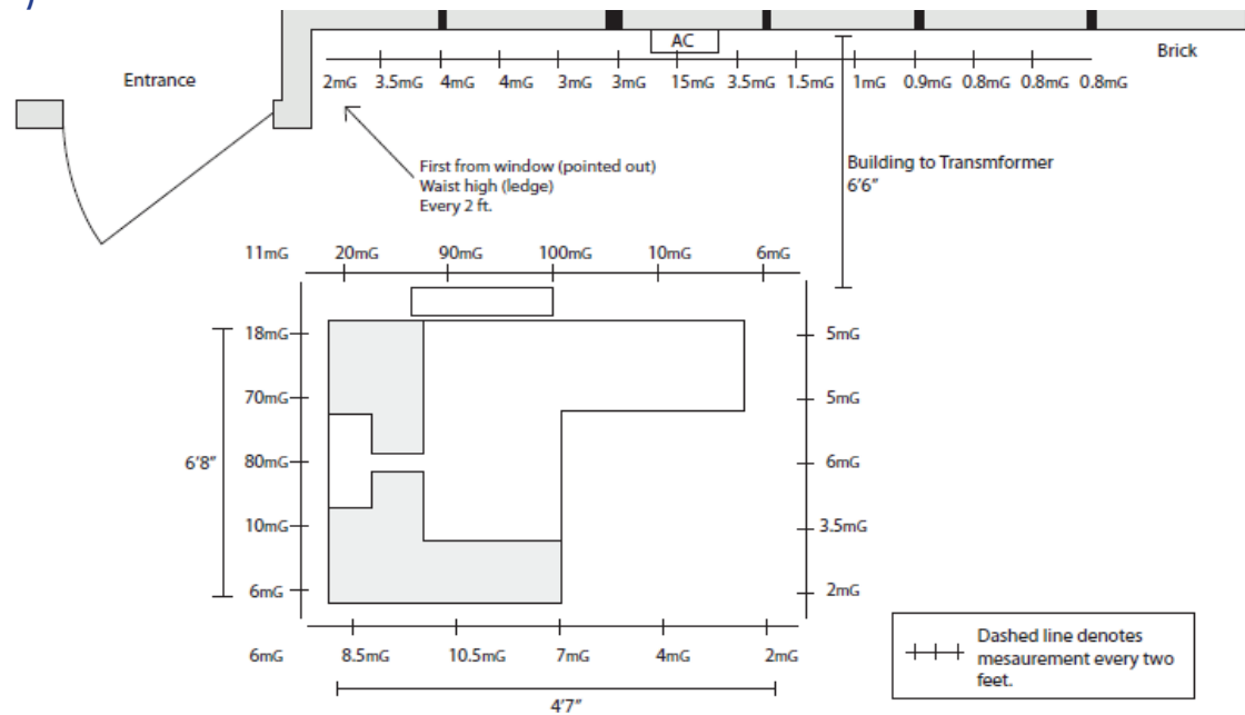
Figure 3. Magnetic field area measurements near transformer and exterior wall of the timekeeping office.
