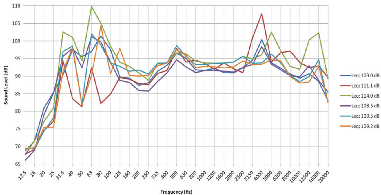
Figure B4. Octave band analysis for necker machines.
