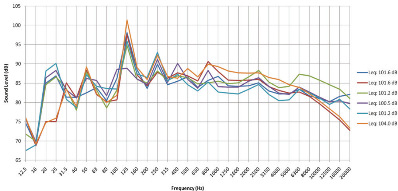
Figure B6. Octave band analysis for baler.
