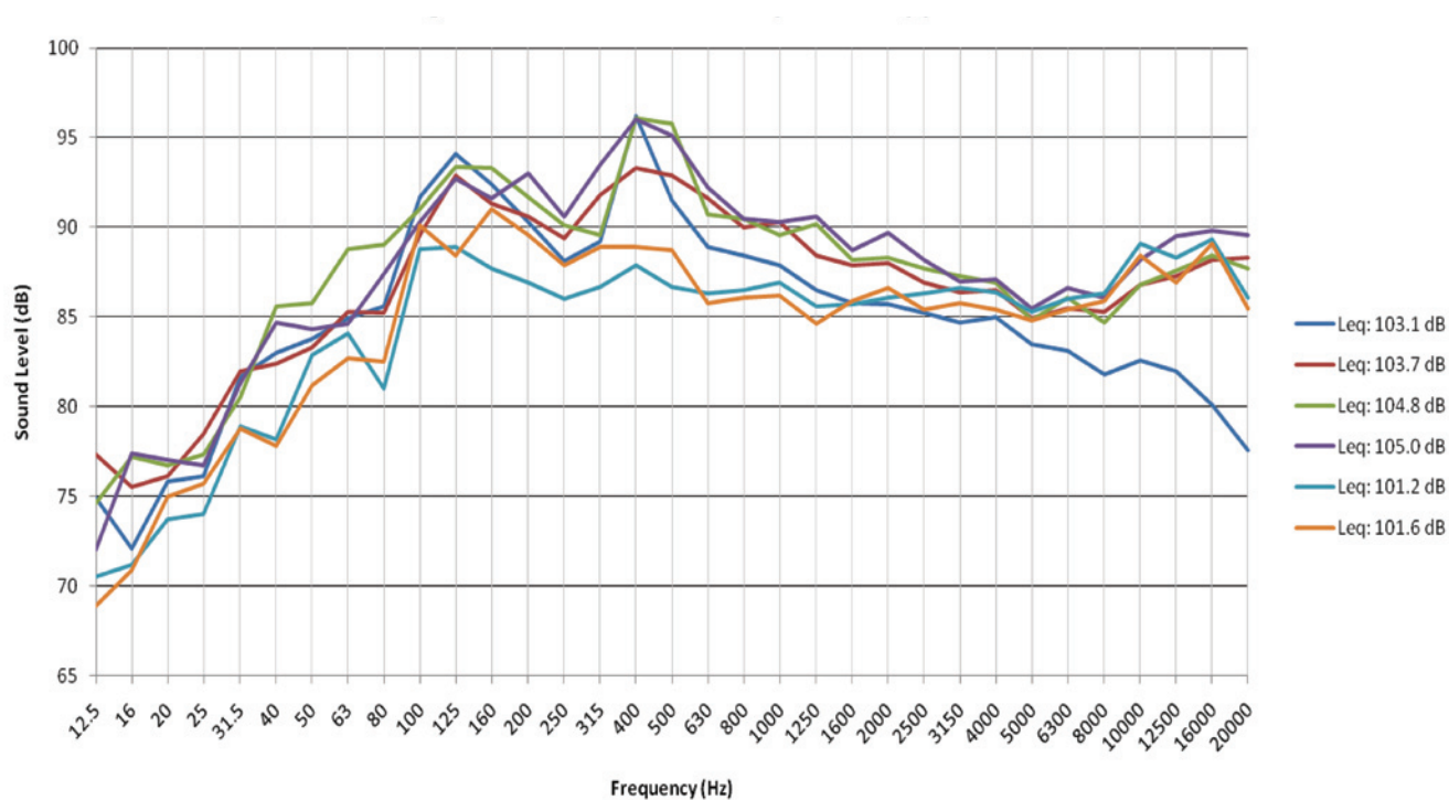
Figure B1. Octave band analysis for copper band press.
