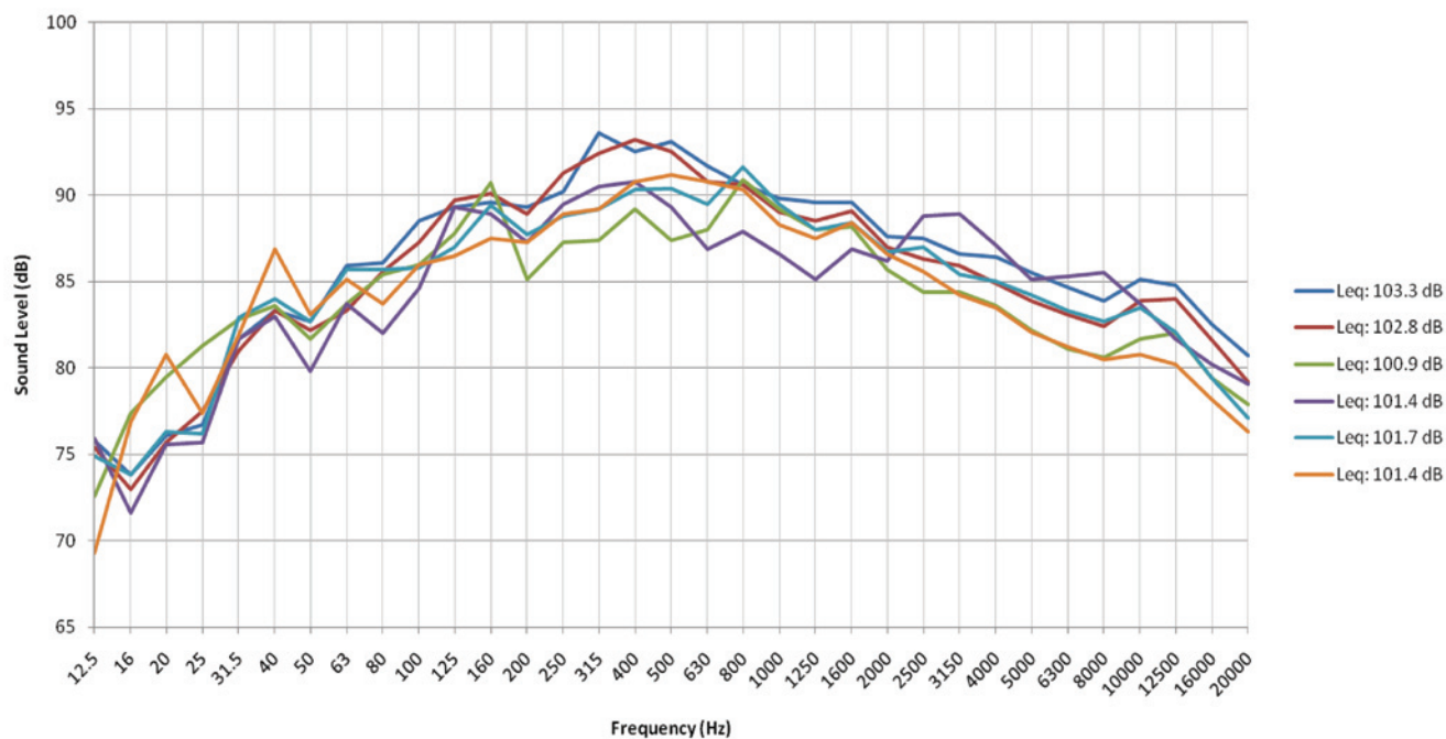
Figure B2. Octave band analysis for ironers.
