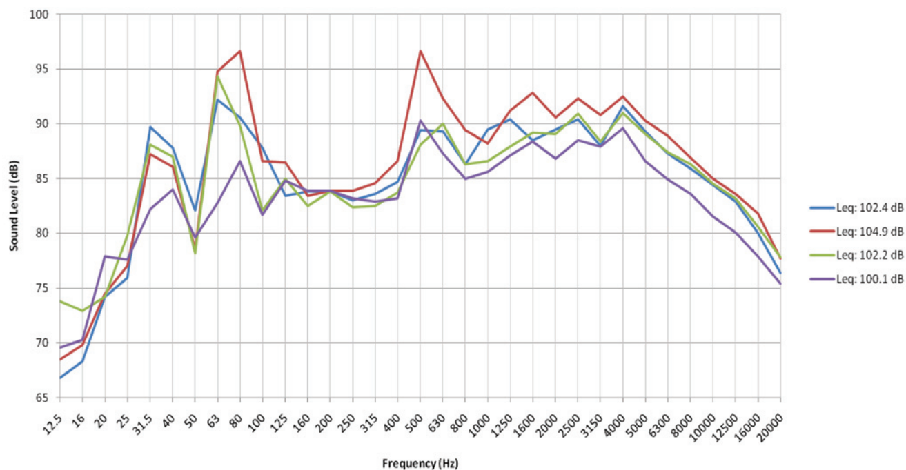
Figure B5. Octave band analysis for lacquer spray machines.
