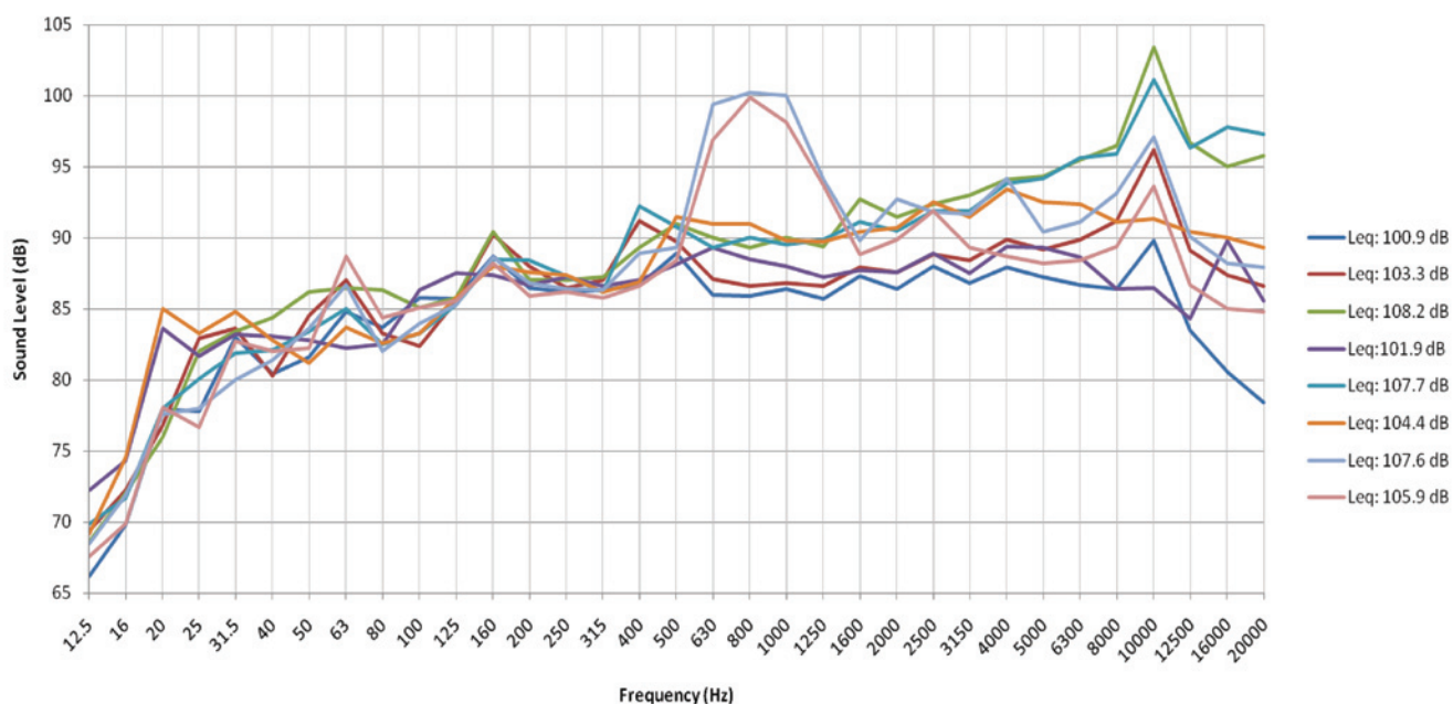
Figure B3. Octave band analysis for printers.
