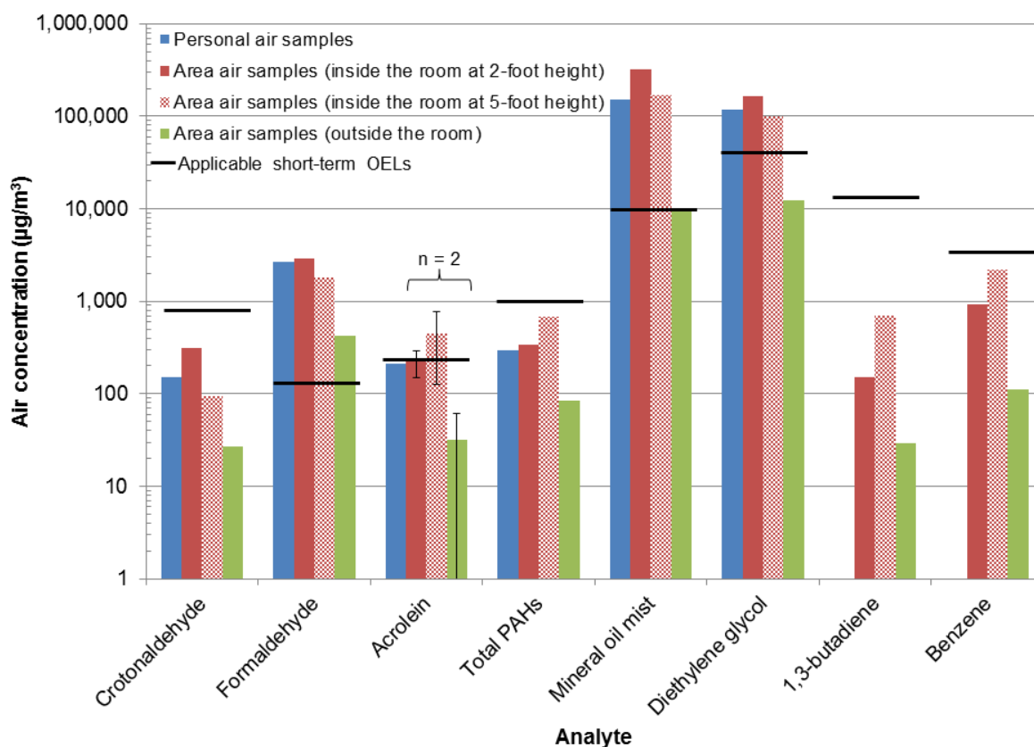
Figure 14. Air concentrations of mineral oil mist, diethylene glycol, and their thermal decomposition products during Exercise 5. Average concentrations and error bars representing the minimum and maximum measurements are provided if more than one sample was collected. If no measurements were collected, then nothing is reported.
