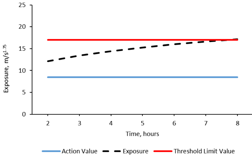
Figure B7. Graph of VDV for up to 8 hours when using the fertilizer equipment.
