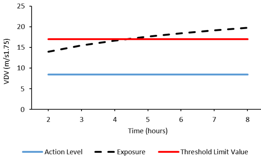
Figure B4. Graph of VDV for up to 8 hours when operating the zero-turn mower.
