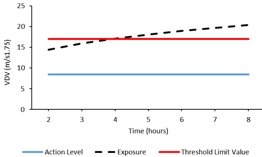
Figure B3. Graph of VDV for up to 8 hours when mowing the tee boxes.
