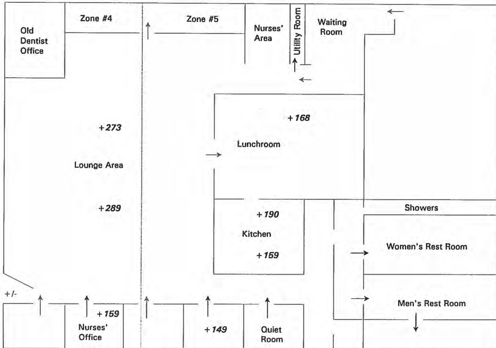
Figure 2 Air Flow Patterns Location: Spectrum Health Care, Inc. Date: March 9-11, 1993 HETA 93-365
