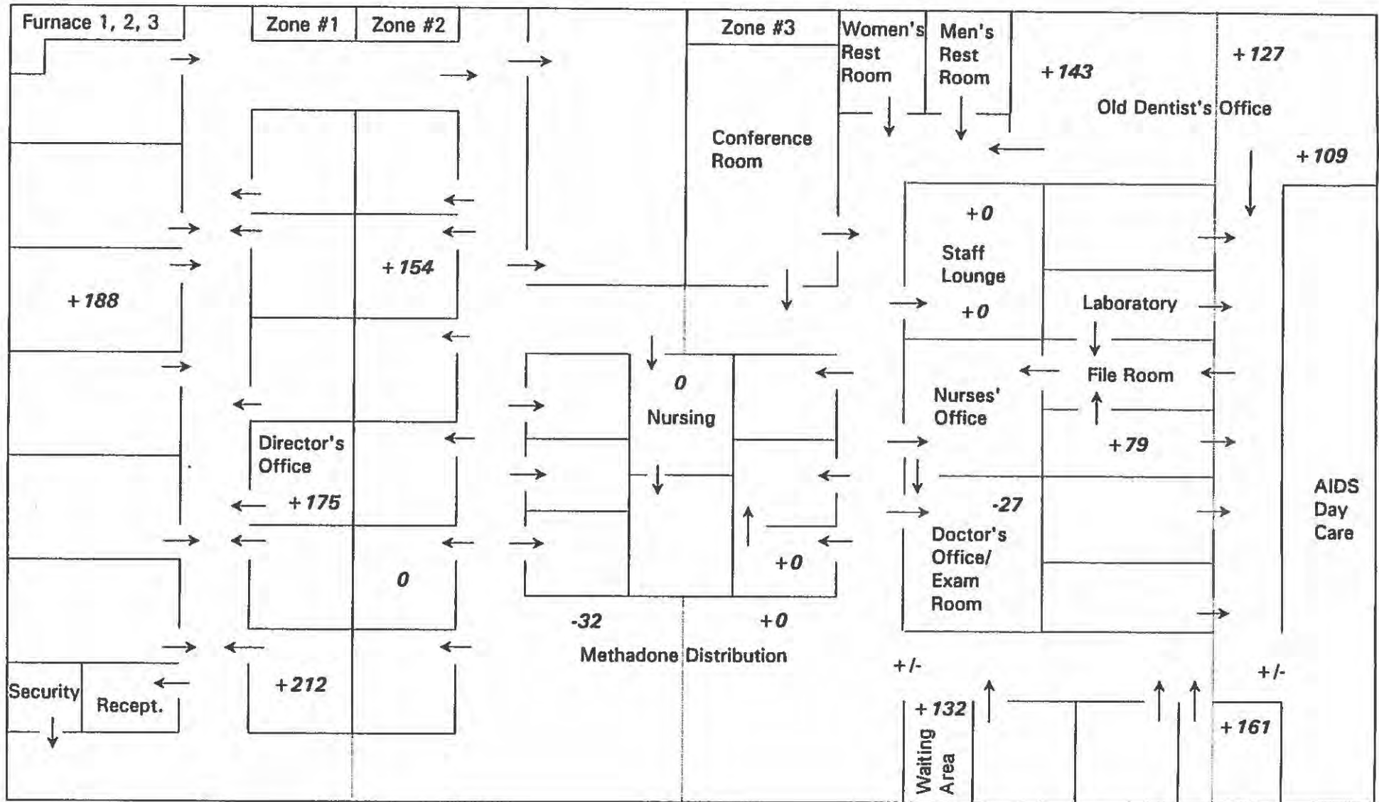
Figure 1 Air Flow Patterns Location: Spectrum Health Care, Inc. Date: March 9-11, 1993 HETA 93-365
