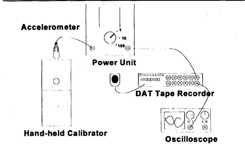
Figure 3: Calibration Set-up
