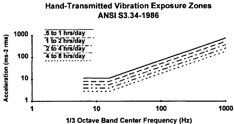
Figure 2: ANSI Recommended HAV Exposure Zones
