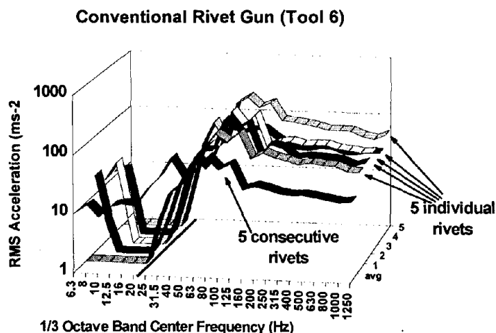
Figure 14: Five Consecutive vs. Five Individual Rivets
