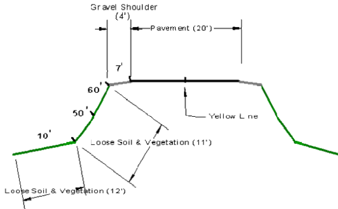
Figure 1. Cross-section of roadway near the incident.
