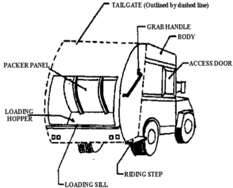
Exhibit 1. A schematic of a rear-loading trash truck.
