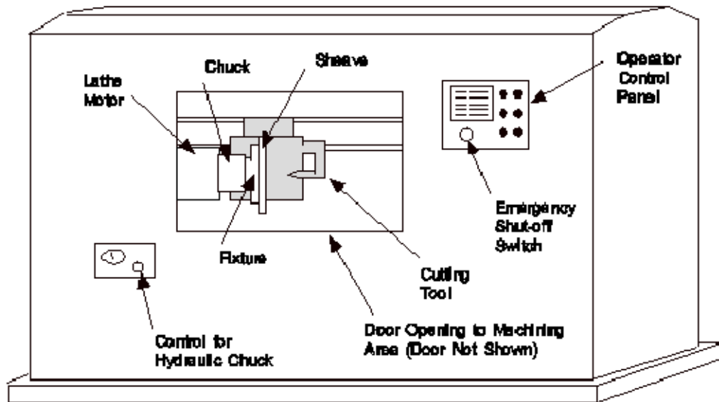
Figure 1. Computer Numeric Controlled (CNC) Lathe (Not to Scale)
