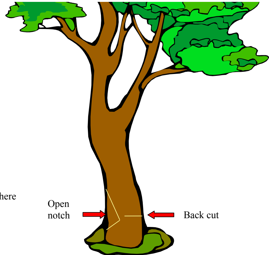
Alternate "Open-Face" Technique
