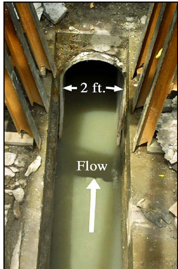
Photo 1 – Bottom of access pit, showing end of liner in narrow duct, direction of sewage flow, and steel legs of overhead tower.
