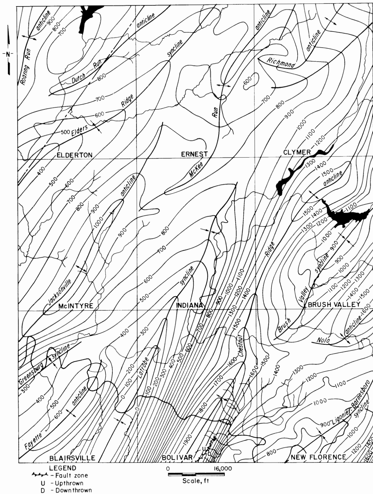
FIGURE 6. - Structure map drawn on the base of the Lower Kittanning coalbed.
