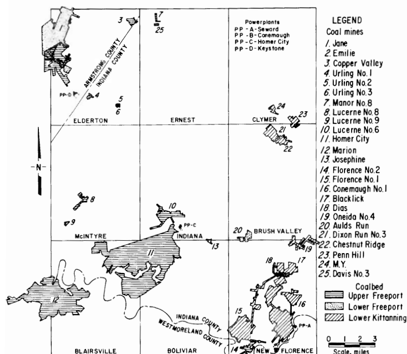
FIGURE 24. - Active underground mines in study area.
