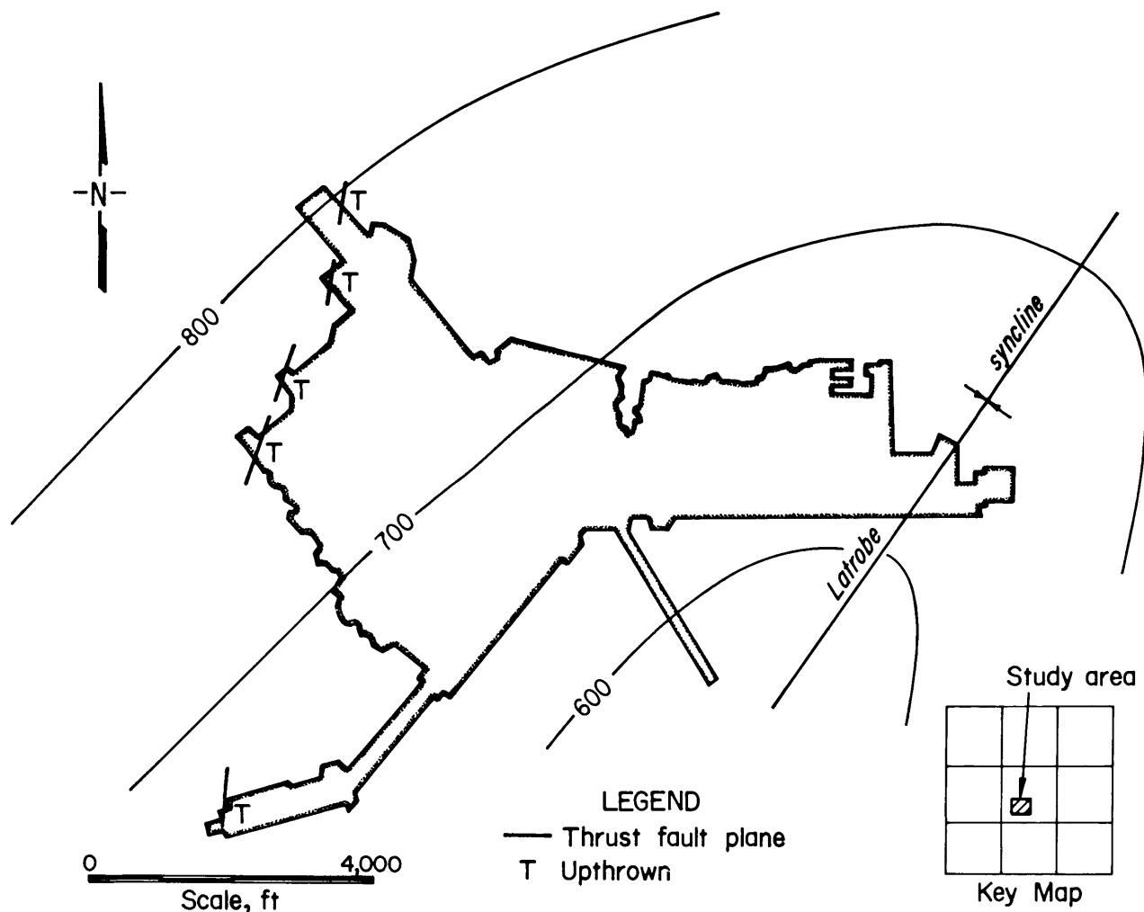
FIGURE 10. - Location of thrust faults in the Lucerne No. 6 mine.
