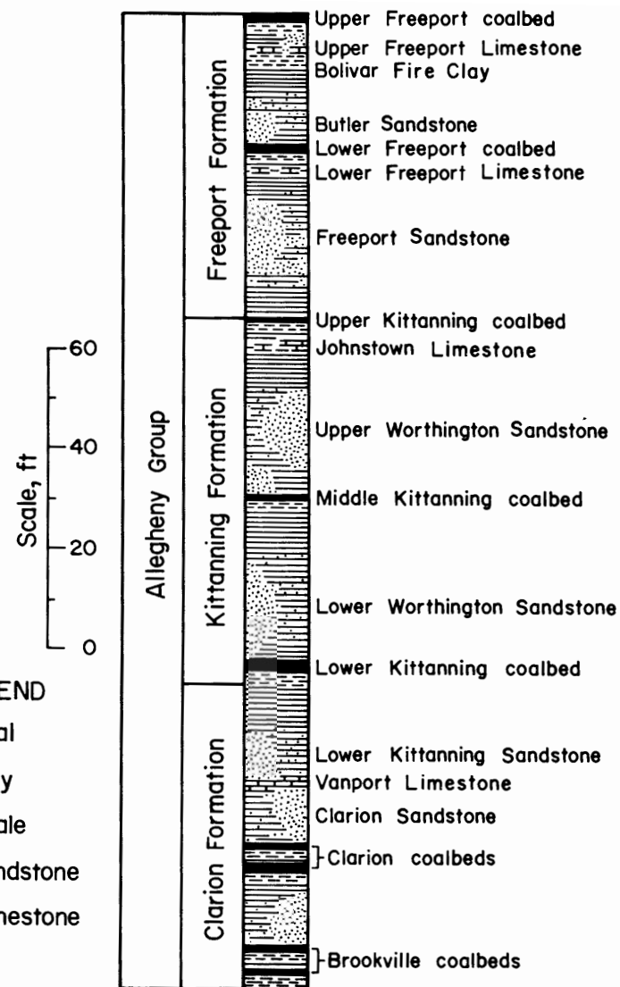
FIGURE 5. - Generalized stratigraphic column of the Allegheny Group.
