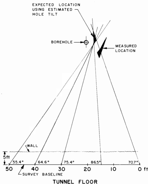
FIGURE B-3. - Effect of coil tilt on location accuracy.
