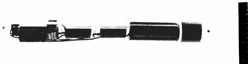
FIGURE 3. - Borehole transmitter.
