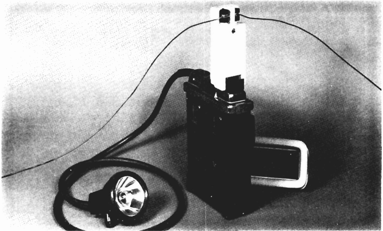
FIGURE 1. - Trapped miner transmitter.
