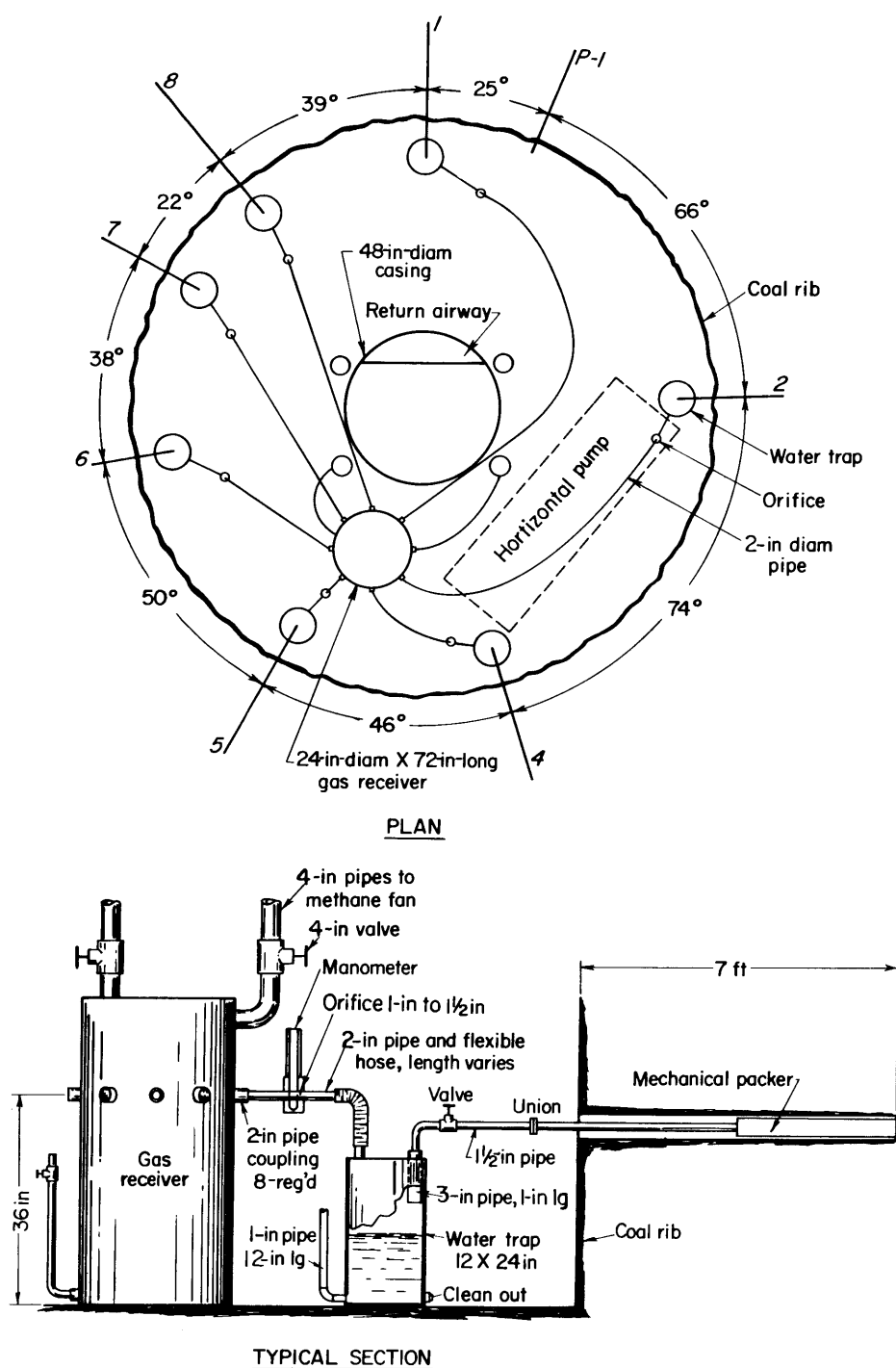
FIGURE 12. - Connection of degasification holes through water traps and receiver tank on bottom.
