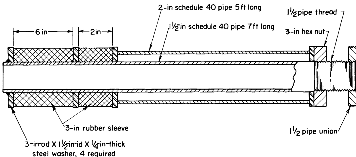
FIGURE 11. - Mechanical packer assembly for holes in coalbed.
