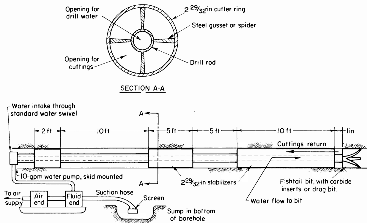
FIGURE 10. - Drilling assembly for holes in coalbed.
