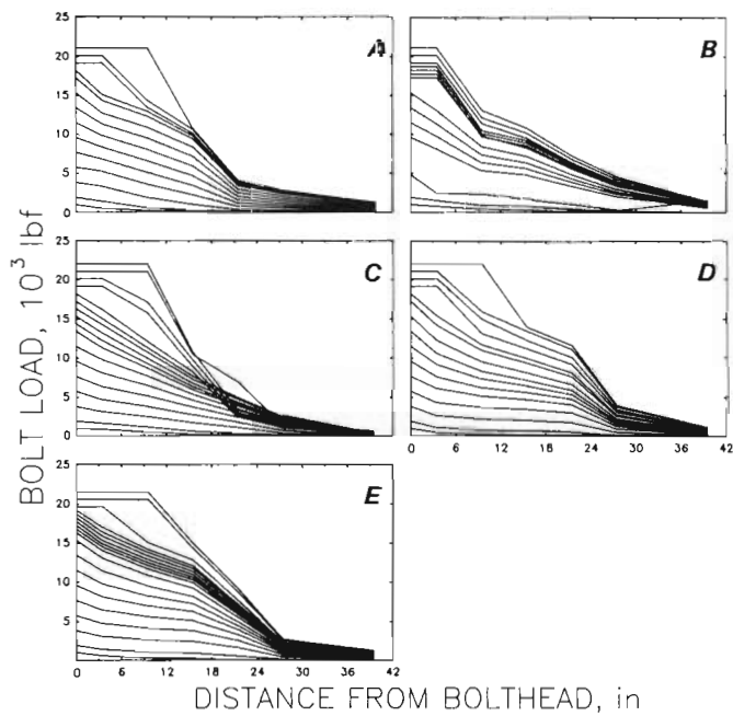
Figure A-5.—Results from plastic test, mine 1. A, Bolt 1; B, bolt 2; C, bolt 3; D, bolt 4; E, bolt 5.
