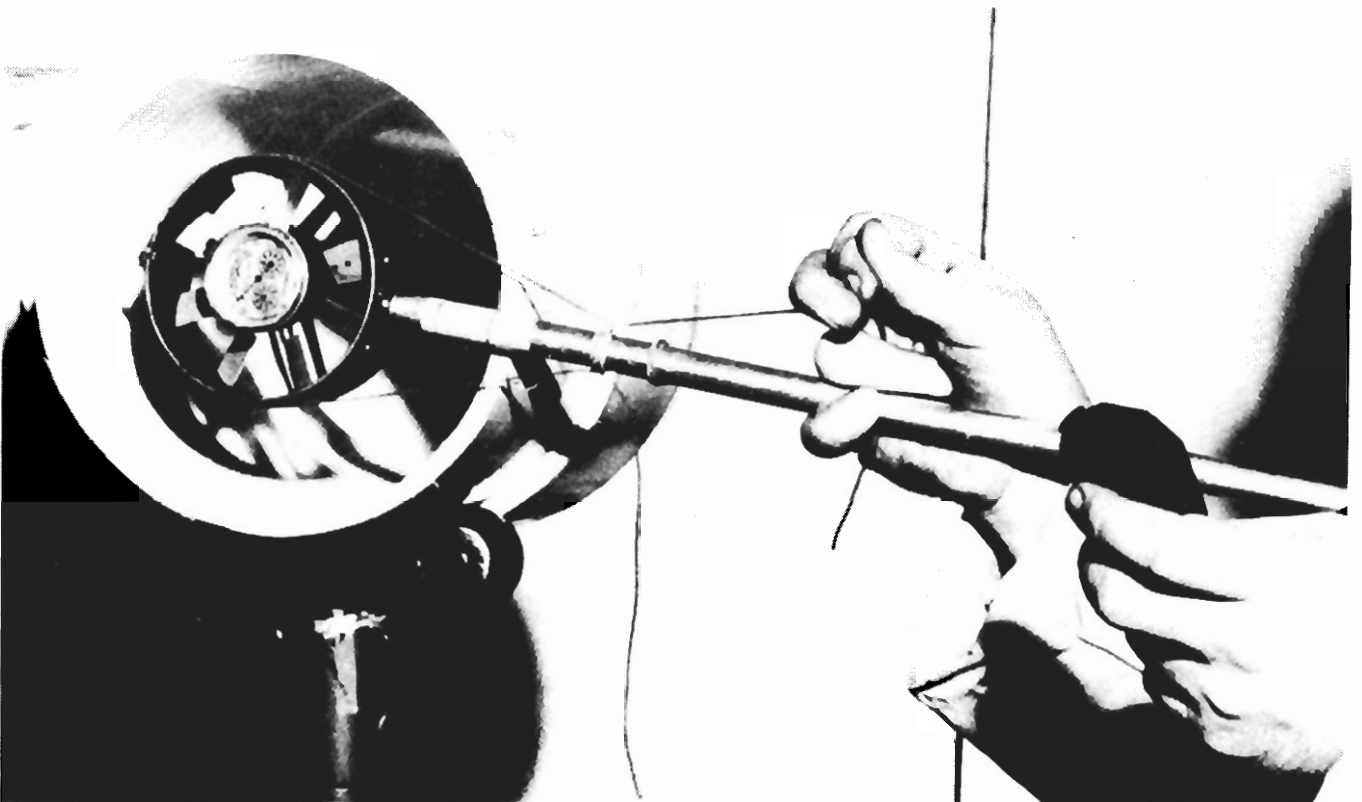
FIGURE 6.—Anemometer measurements closer than 7.5 pipe diameters from an elbow.
