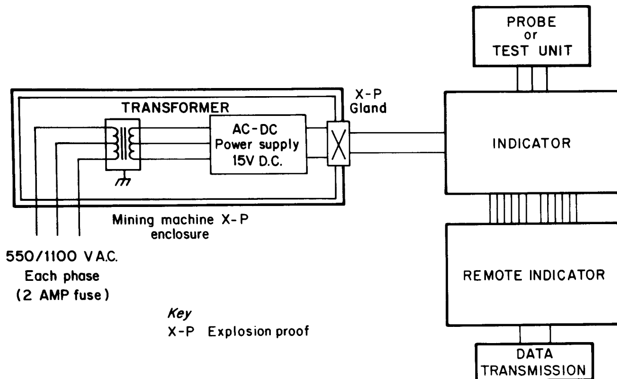
Block diagram for RHC 801 natural gamma coal thickness indication system.
