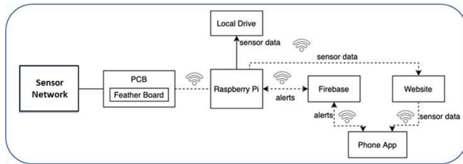
Figure 14. Architecture of the Continuous Fit Monitoring System.
