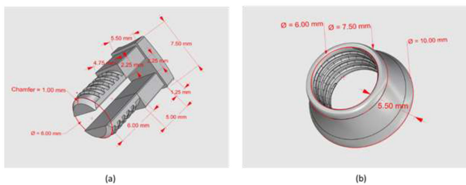
Figure 10. Design and dimensions of the Screw Peg and Cap. (a) Screw Peg. (b) Screw Cap.
