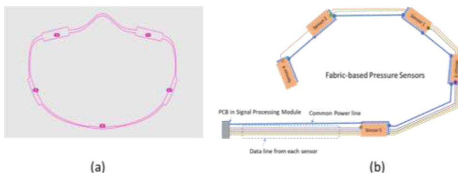
Figure 2. Continuous Fit Monitoring Sensor Network and Locations in RPD Frame. (a) Locations of sensor for the continuous fit monitoring system in RPD frame. (b) Schematic of continuous fit monitoring sensor network system.
