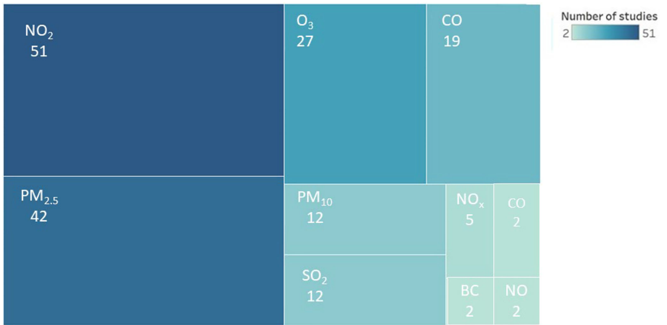
Fig. 2. A thematic map of number of studies included in this scoping review, by air pollutants. Studies could examine more than one pollutant. The numbers reflect the total number of studies that examined a particular pollutant.
