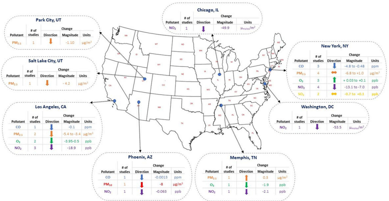
Fig. 3. Location-specific summary of magnitude and direction of change in air pollutants.
