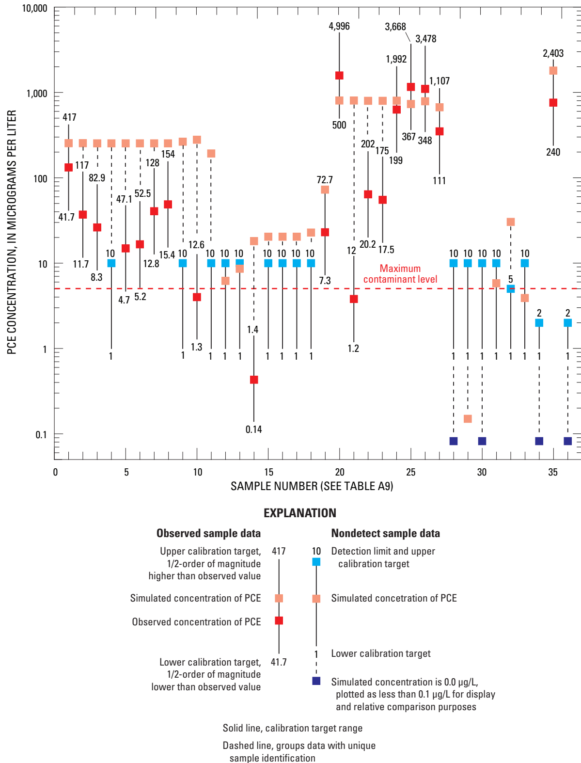
Figure A11. Comparison of observed and nondetect tetrachloroethylene sample data with calibration targets and simulated concentrations at water-supply wells, Tarawa Terrace, U.S. Marine Corps Base Camp Lejeune, North Carolina. [PCE, tetrachloroethylene; µg/L, microgram per liter]
