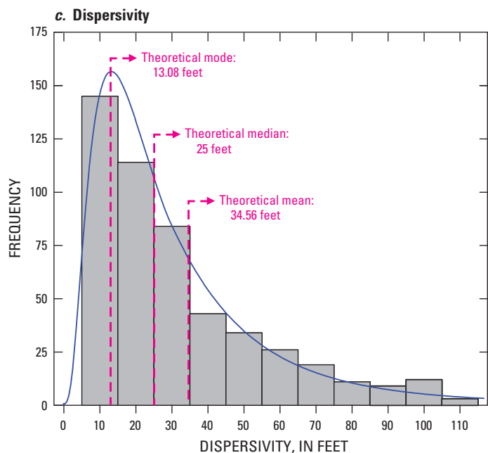
Figure A23. Probability density functions for (a) recharge rate, (b) mass loading rate (source concentration), and (c) dispersivity used to conduct probabilistic analyses. [-, minus; +, plus]
