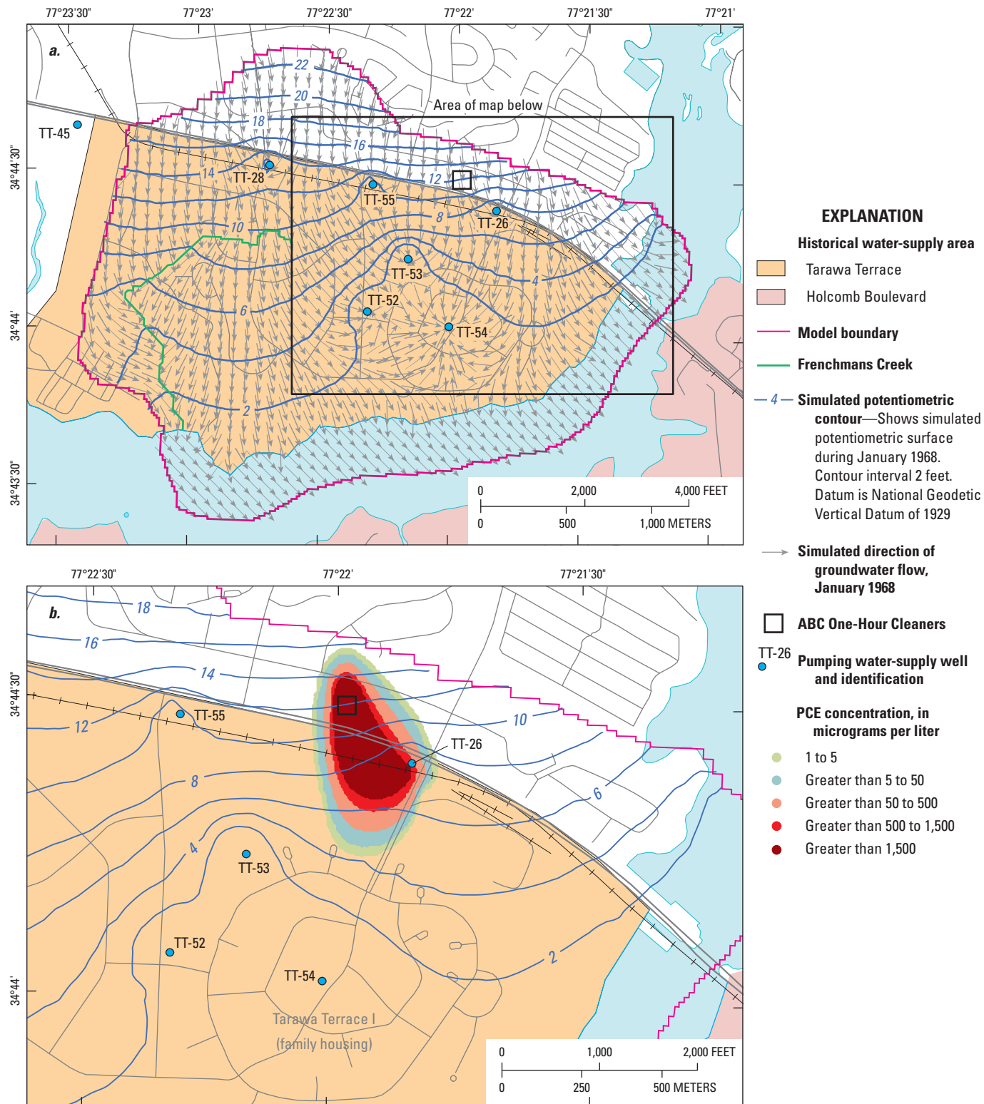
Figure A14. Simulated (a) water level and direction of groundwater flow and (b) distribution of tetrachloroethylene, model layer 1, January 1968, Tarawa Terrace and vicinity, U.S. Marine Corps Base Camp Lejeune, North Carolina. [PCE, tetrachloroethylene]
