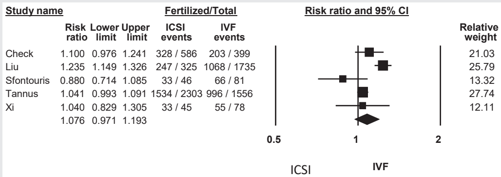
Forest plot presenting risk ratios for fertilization with intracytoplasmic sperm injection (ICSI) compared to conventional in vitro fertilization (IVF) among women of advanced age with non-male factor infertility using only MII mature oocytes. Meta-analysis using random effects model. Q = 19.6, P < .001, I^2 = 79.6 .
