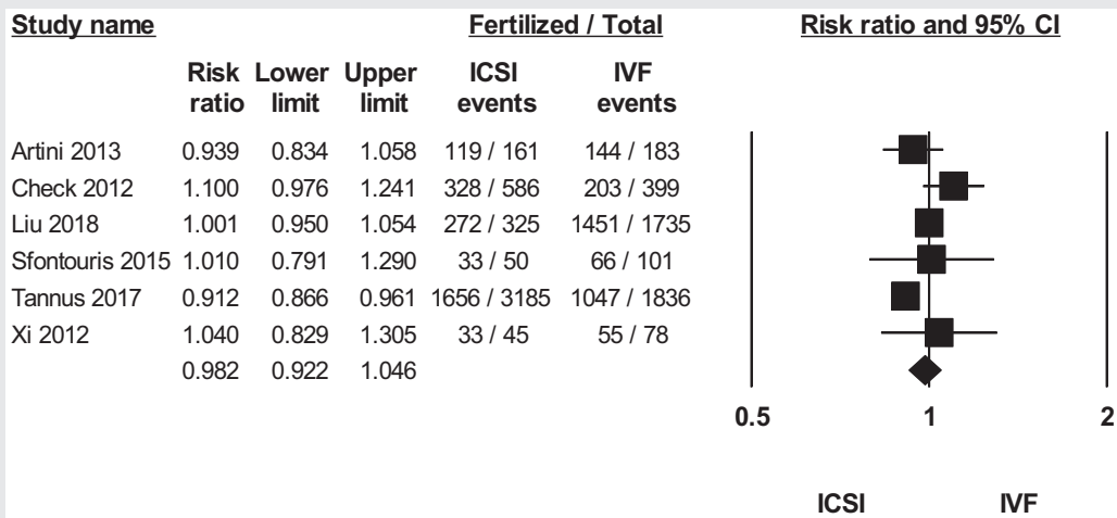
Forest plot presenting risk ratios for fertilization with intracytoplasmic sperm injection (ICSI) compared to conventional in vitro fertilization (IVF) among women of advanced age with non-male factor infertility with no prior fertilization failure. Meta-analysis using random effects model. Q = 11.7, P < .05, I^2 = 57.1 .
