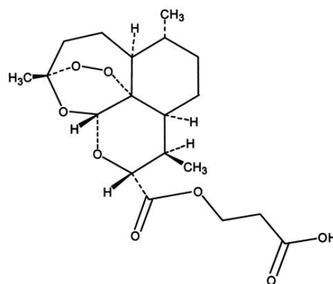
Artesunate
