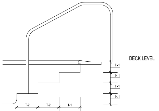
Figure 4.5.4.5.2: Stair Treads: Front View
