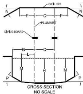
Figure 4.8.2.2.2: Diving Platform Cross Section: Front View
