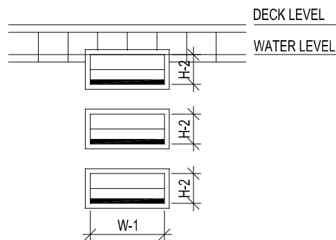
Figure 4.5.7.4.2: Recessed Step Dimensions: Front View
