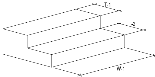
Figure 4.5.4.5.3: Unique Stair Treads
