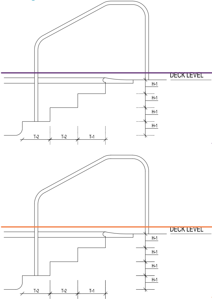
Figure 4.5.4.5.1: Stair Treads and Risers
