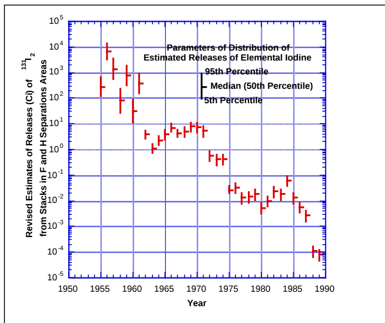
Figure 1-7. RAC releases estimates of ^{131}\text{I} in elemental form ( \text{I}_2 ) from stacks in the F and H separations areas. For each year, the length of the vertical line shows the range (5 th to 95 th percentiles ) of the distribution of release estimates and the median estimate is indicated by the horizontal bar.
