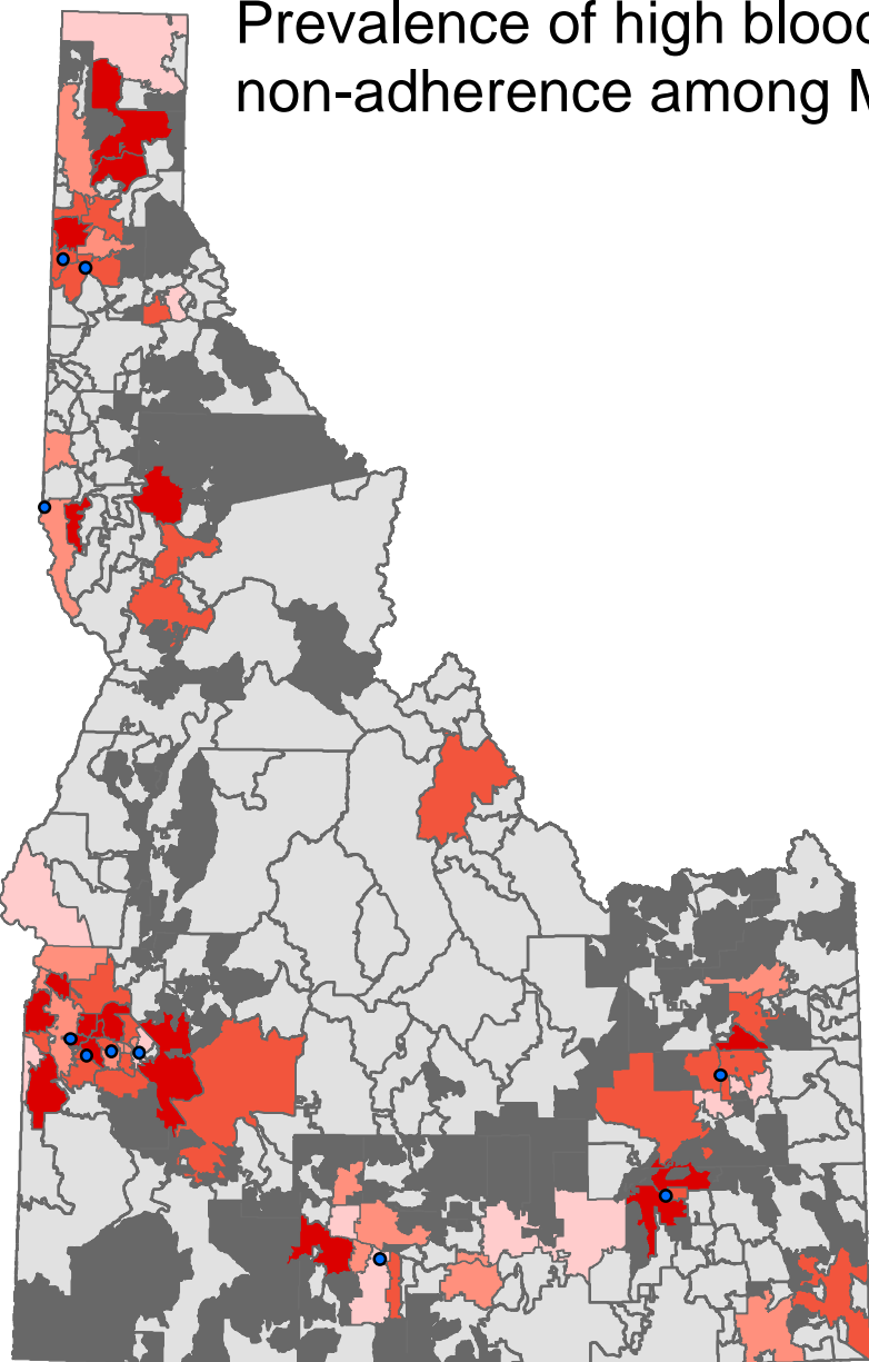
ZCTA Only
