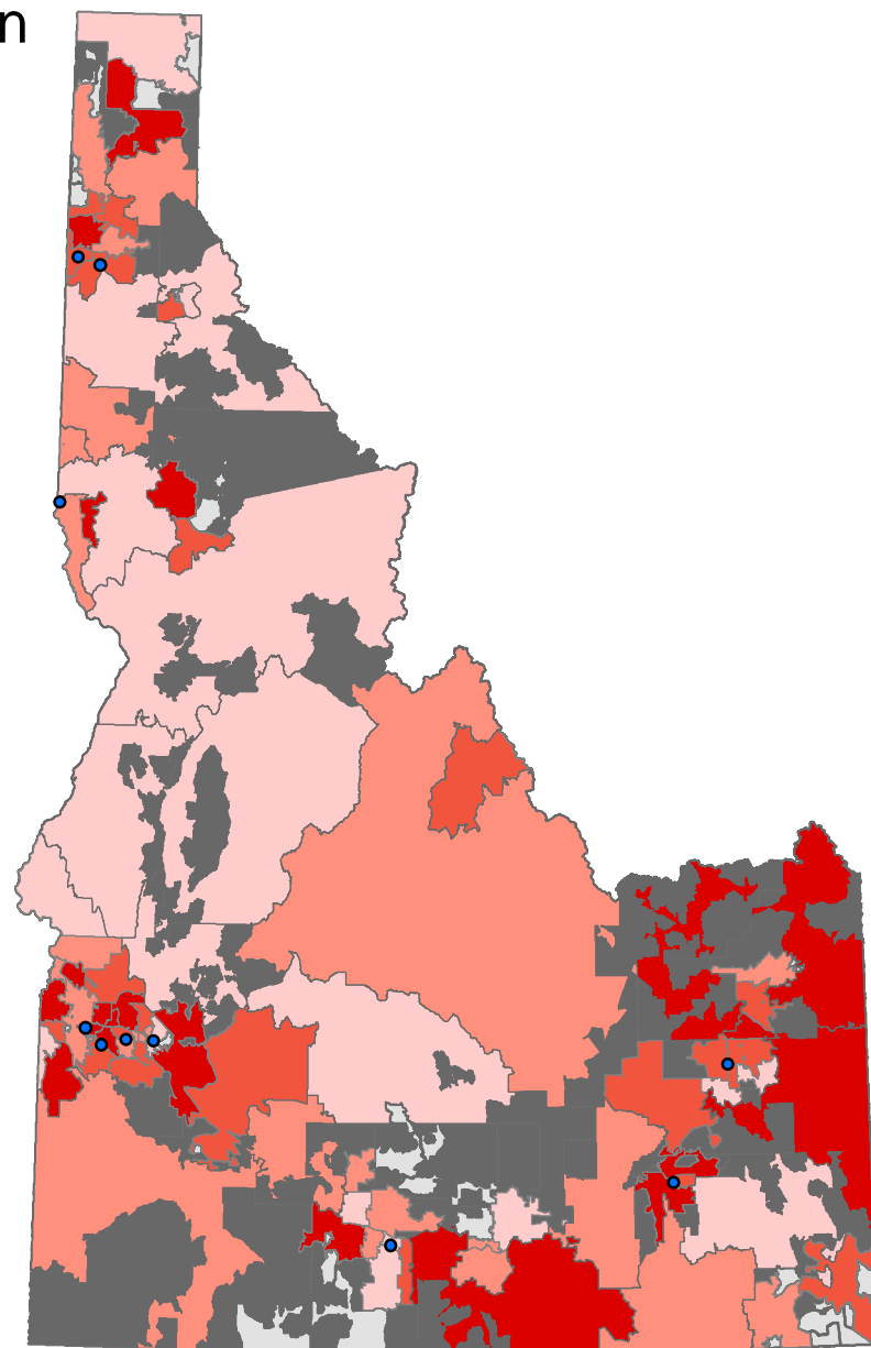
ZCTA/ZCTA Groups
