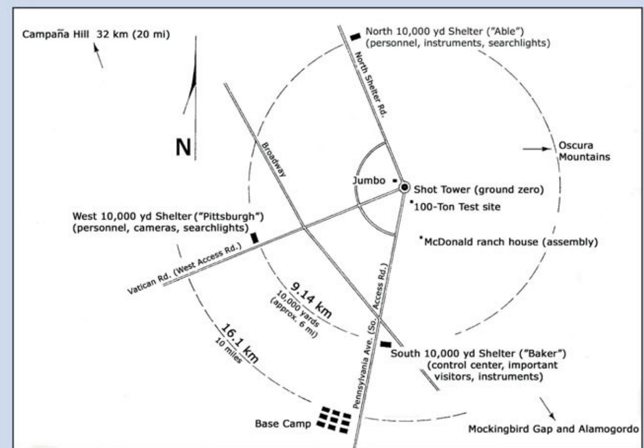
Fig. 1. Layout of the Trinity Test Site near Socorro, New Mexico
