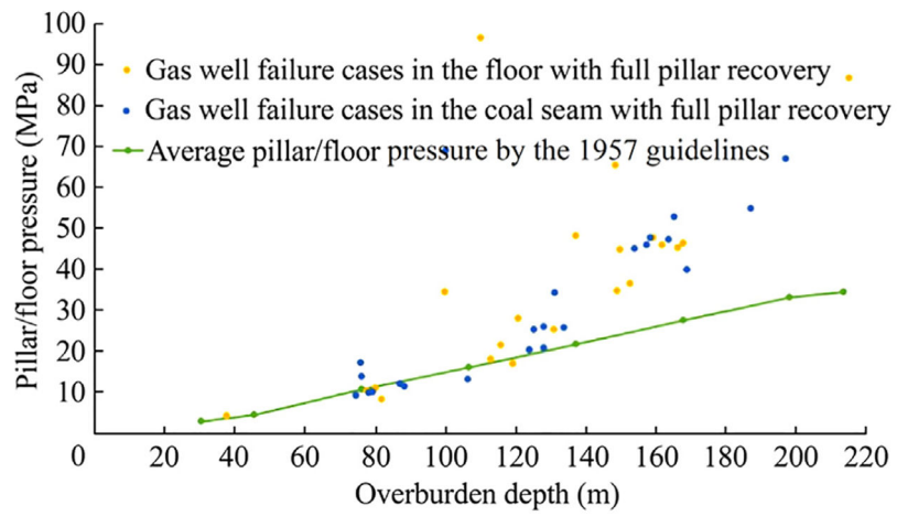
Fig. 10. Calculated average pillar/floor pressure for the pillars by the 1957 guidelines in comparison with the calculated pillar/floor pressure for the failure cases in the coal seam and floor.
