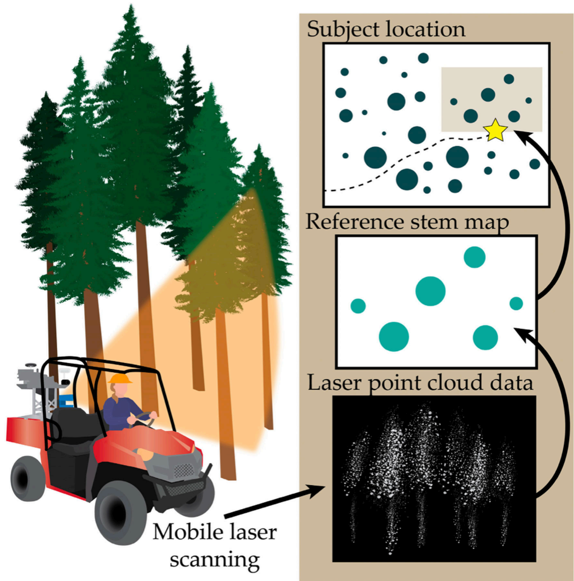
Figure 7. Simultaneous Location and Mapping (SLAM) techniques in the forest (based on Qian et al.) [7]. First, reference trees with known diameters must be mapped with their GNSS coordinates (not shown). Then, mobile laser scanning equipment (e.g., LiDAR) scans an area of interest in the woods ( left ). From the LiDAR point cloud data ( bottom right ), a stem distribution map is generated (middle right), which is compared to the reference tree map ( top right ) and in turn used to determine position. In practice, certainty in the map and location estimates improves with repeated passes and multiple perspectives.
